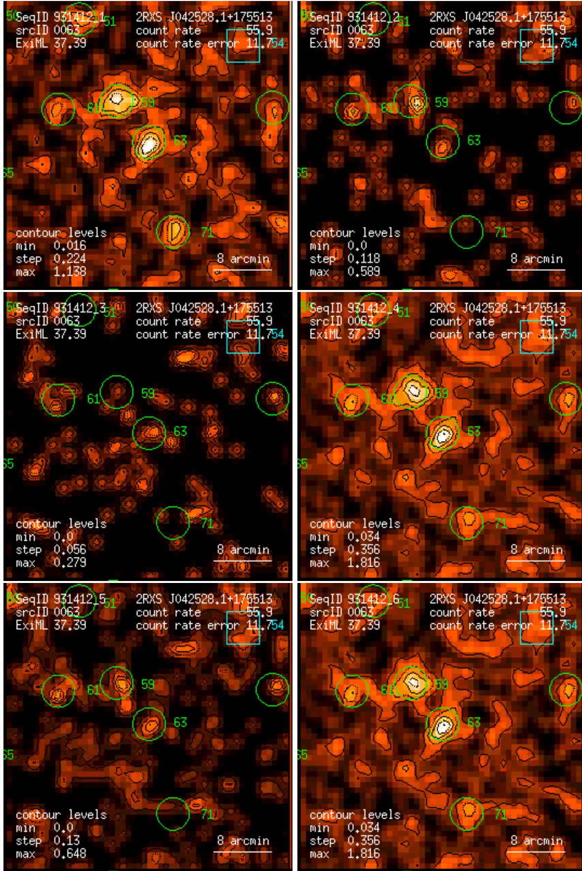
Figure 63: RASS 931412: detection 0063: band rate images, Gaussian filter: (1) PSPC channels 11 – 41, (2) 52 – 90, (3) 91 – 201, (4) 11 – 235, (5) 52 – 201, (6) 11 – 201. Broad band rates in counts/ks. Band rate contour levels in counts/ks/arcmin 2 .
