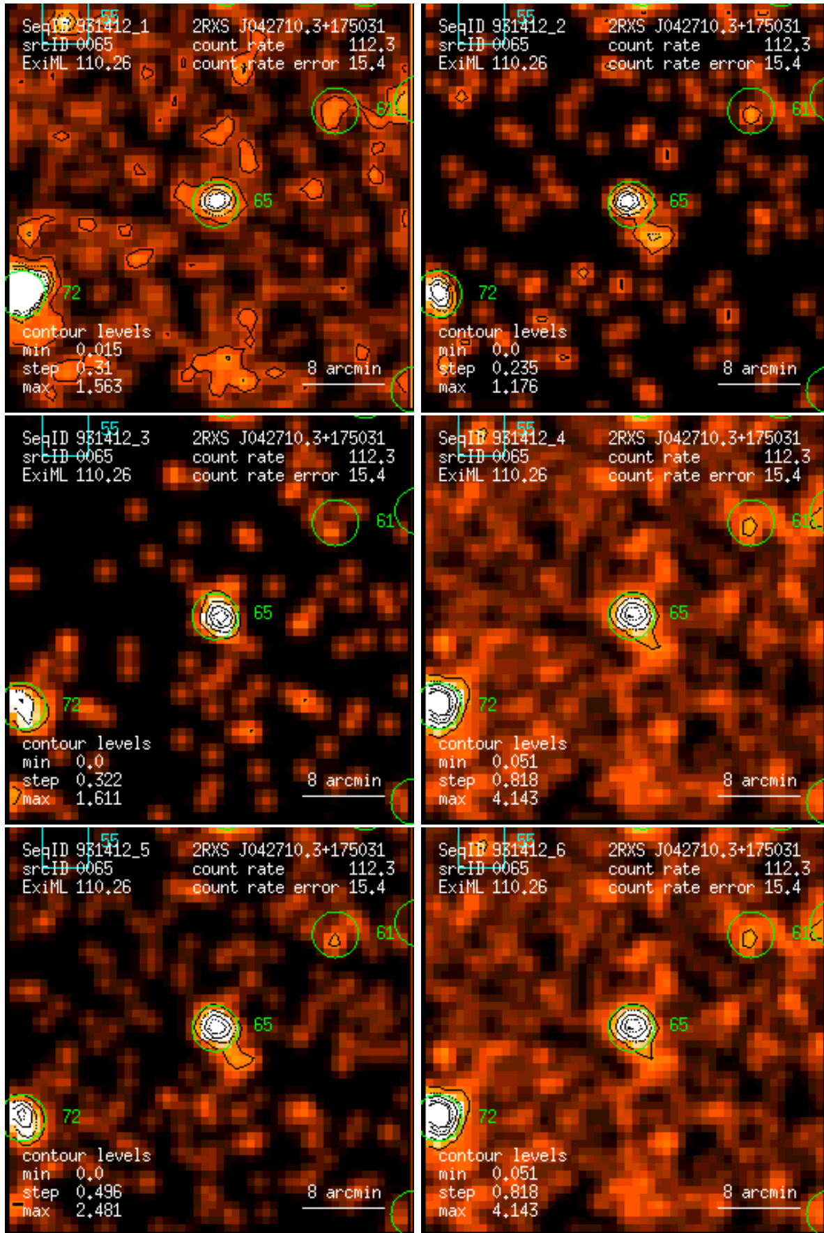
Figure 65: RASS 931412: detection 0065: band rate images, Gaussian filter: (1) PSPC channels 11 – 41, (2) 52 – 90, (3) 91 – 201, (4) 11 – 235, (5) 52 – 201, (6) 11 – 201. Broad band rates in counts/ks. Band rate contour levels in counts/ks/arcmin 2 .
