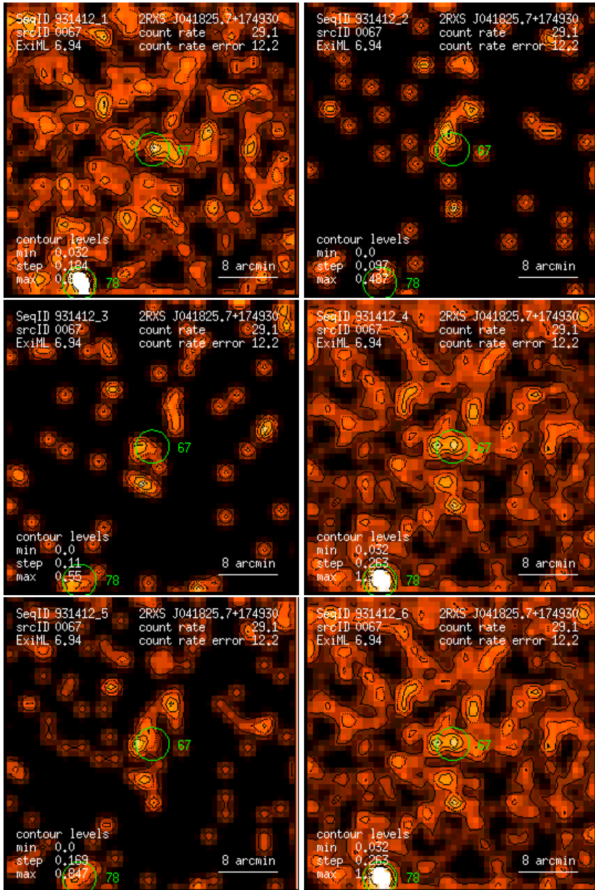
Figure 67: RASS 931412: detection 0067: band rate images, Gaussian filter: (1) PSPC channels 11 – 41, (2) 52 – 90, (3) 91 – 201, (4) 11 – 235, (5) 52 – 201, (6) 11 – 201. Broad band rates in counts/ks. Band rate contour levels in counts/ks/arcmin 2 .
