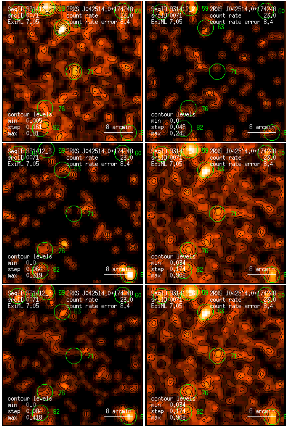
Figure 71: RASS 931412: detection 0071: band rate images, Gaussian filter: (1) PSPC channels 11 – 41, (2) 52 – 90, (3) 91 – 201, (4) 11 – 235, (5) 52 – 201, (6) 11 – 201. Broad band rates in counts/ks. Band rate contour levels in counts/ks/arcmin 2 .
