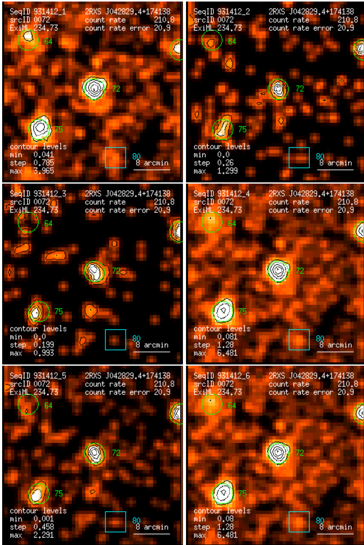
Figure 72: RASS 931412: detection 0072: band rate images, Gaussian filter: (1) PSPC channels 11 – 41, (2) 52 – 90, (3) 91 – 201, (4) 11 – 235, (5) 52 – 201, (6) 11 – 201. Broad band rates in counts/ks. Band rate contour levels in counts/ks/arcmin 2 .
