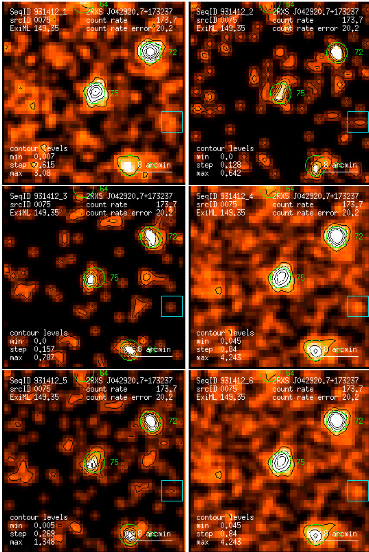
Figure 75: RASS 931412: detection 0075: band rate images, Gaussian filter: (1) PSPC channels 11 – 41, (2) 52 – 90, (3) 91 – 201, (4) 11 – 235, (5) 52 – 201, (6) 11 – 201. Broad band rates in counts/ks. Band rate contour levels in counts/ks/arcmin 2 .
