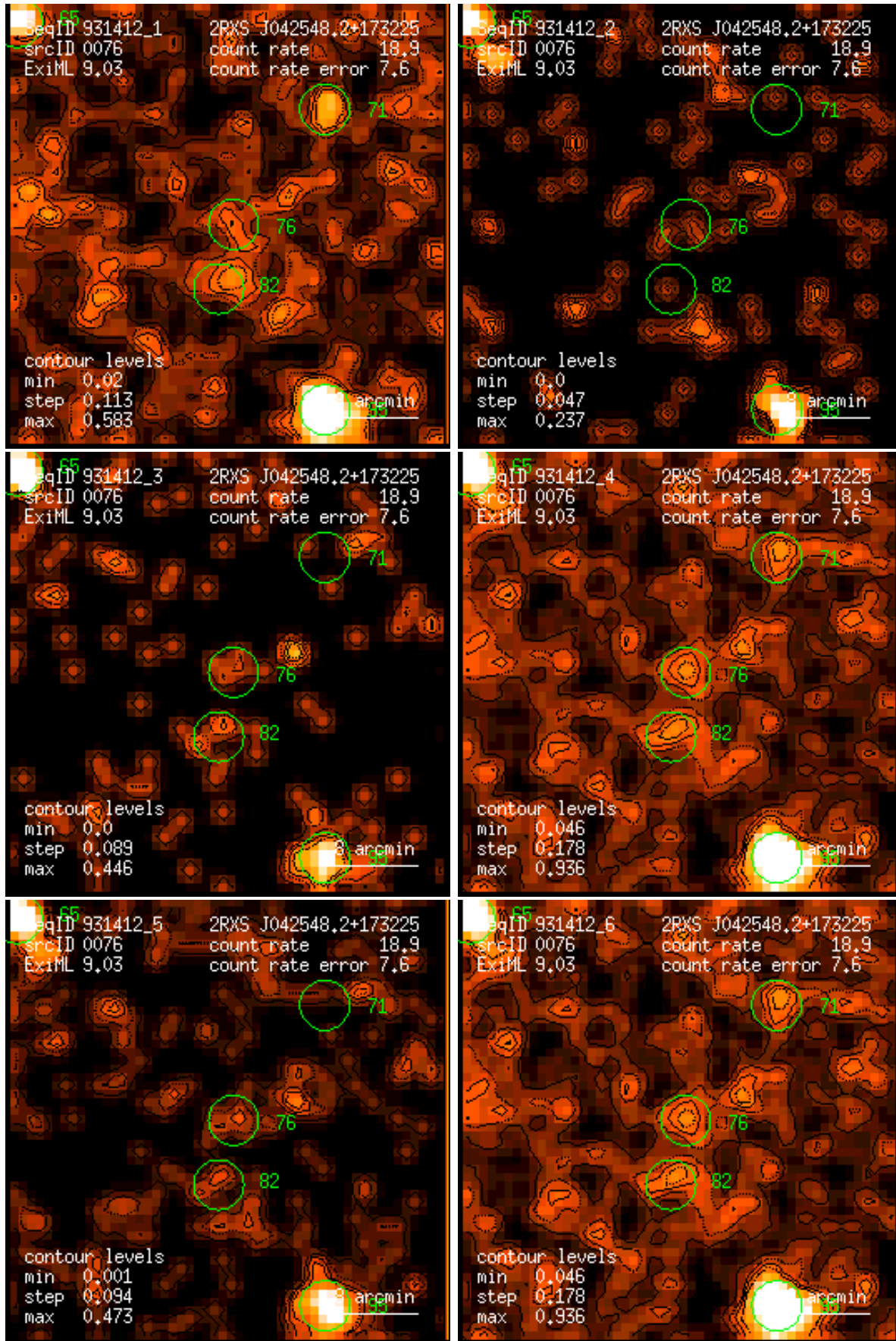
Figure 76: RASS 931412: detection 0076: band rate images, Gaussian filter: (1) PSPC channels 11 – 41, (2) 52 – 90, (3) 91 – 201, (4) 11 – 235, (5) 52 – 201, (6) 11 – 201. Broad band rates in counts/ks. Band rate contour levels in counts/ks/arcmin 2 .
