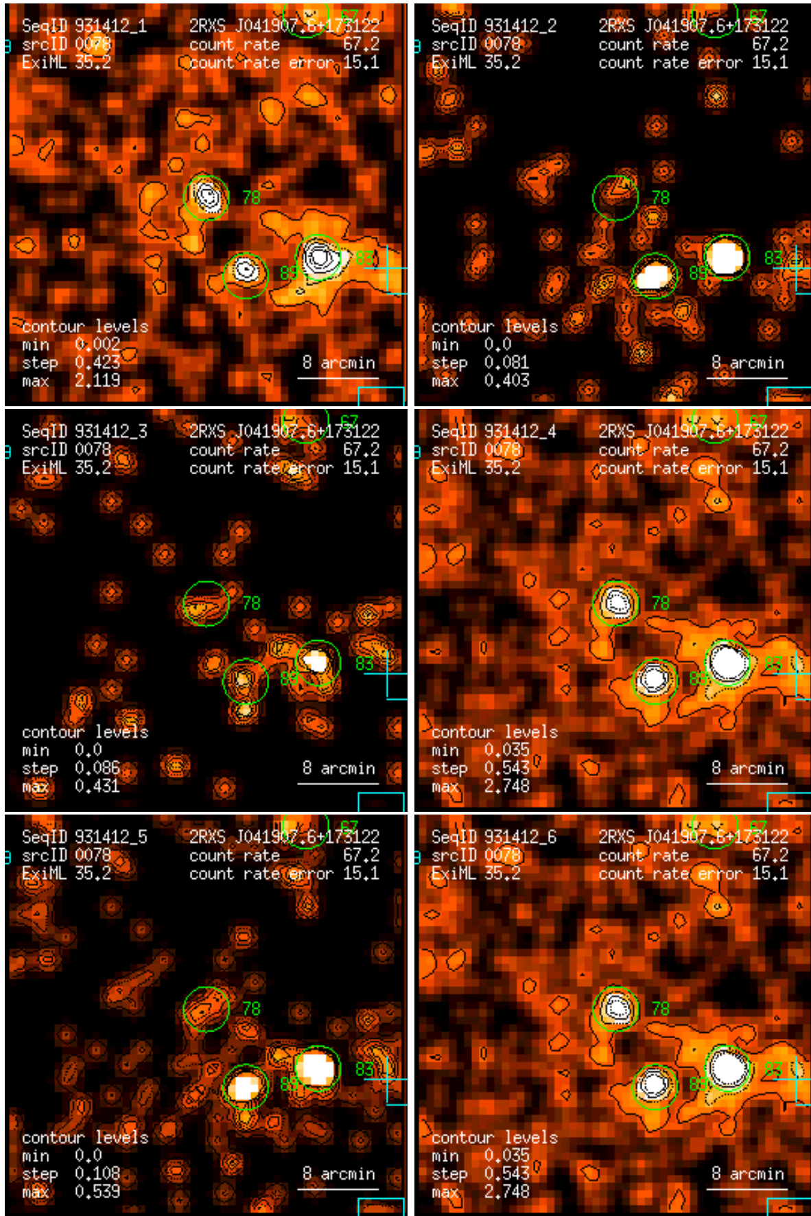
Figure 78: RASS 931412: detection 0078: band rate images, Gaussian filter: (1) PSPC channels 11 – 41, (2) 52 – 90, (3) 91 – 201, (4) 11 – 235, (5) 52 – 201, (6) 11 – 201. Broad band rates in counts/ks. Band rate contour levels in counts/ks/arcmin 2 .
