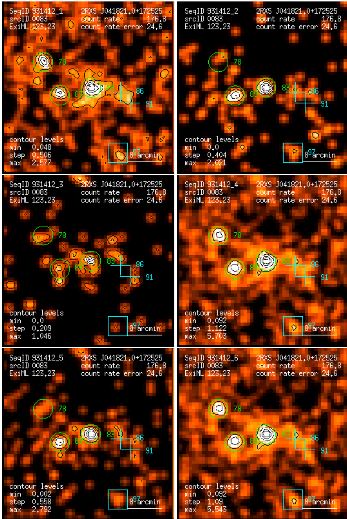
Figure 83: RASS 931412: detection 0083: band rate images, Gaussian filter: (1) PSPC channels 11 – 41, (2) 52 – 90, (3) 91 – 201, (4) 11 – 235, (5) 52 – 201, (6) 11 – 201. Broad band rates in counts/ks. Band rate contour levels in counts/ks/arcmin 2 .
