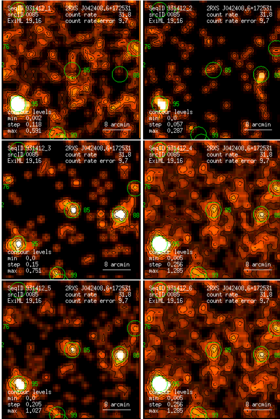
Figure 85: RASS 931412: detection 0085: band rate images, Gaussian filter: (1) PSPC channels 11 – 41, (2) 52 – 90, (3) 91 – 201, (4) 11 – 235, (5) 52 – 201, (6) 11 – 201. Broad band rates in counts/ks. Band rate contour levels in counts/ks/arcmin 2 .
