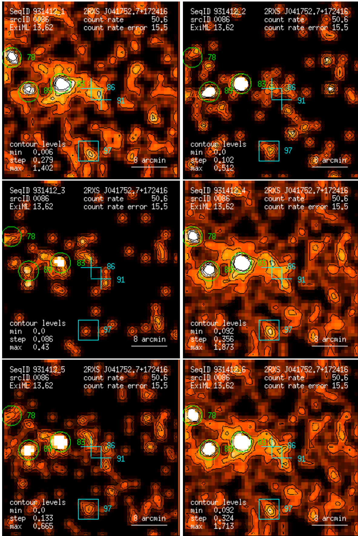
Figure 86: RASS 931412: detection 0086: band rate images, Gaussian filter: (1) PSPC channels 11 – 41, (2) 52 – 90, (3) 91 – 201, (4) 11 – 235, (5) 52 – 201, (6) 11 – 201. Broad band rates in counts/ks. Band rate contour levels in counts/ks/arcmin 2 .
