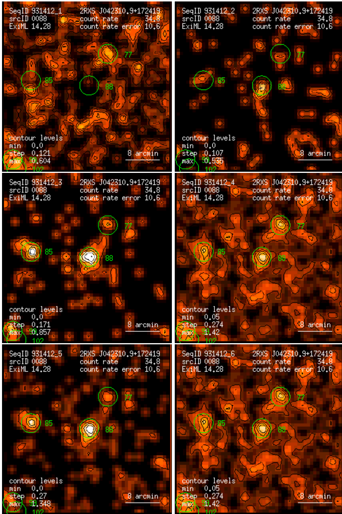
Figure 88: RASS 931412: detection 0088: band rate images, Gaussian filter: (1) PSPC channels 11 – 41, (2) 52 – 90, (3) 91 – 201, (4) 11 – 235, (5) 52 – 201, (6) 11 – 201. Broad band rates in counts/ks. Band rate contour levels in counts/ks/arcmin 2 .
