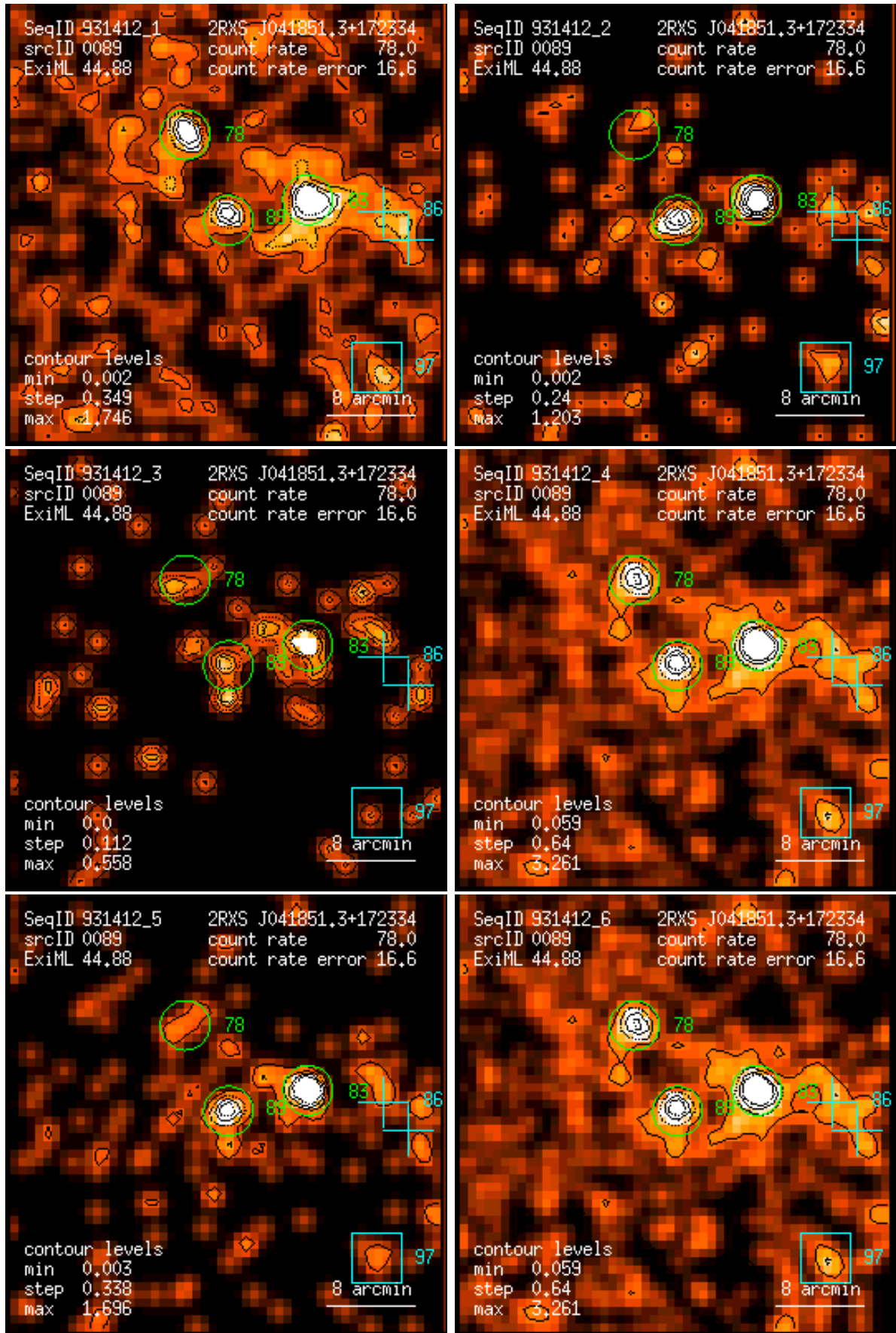
Figure 89: RASS 931412: detection 0089: band rate images, Gaussian filter: (1) PSPC channels 11 – 41, (2) 52 – 90, (3) 91 – 201, (4) 11 – 235, (5) 52 – 201, (6) 11 – 201. Broad band rates in counts/ks. Band rate contour levels in counts/ks/arcmin 2 .
