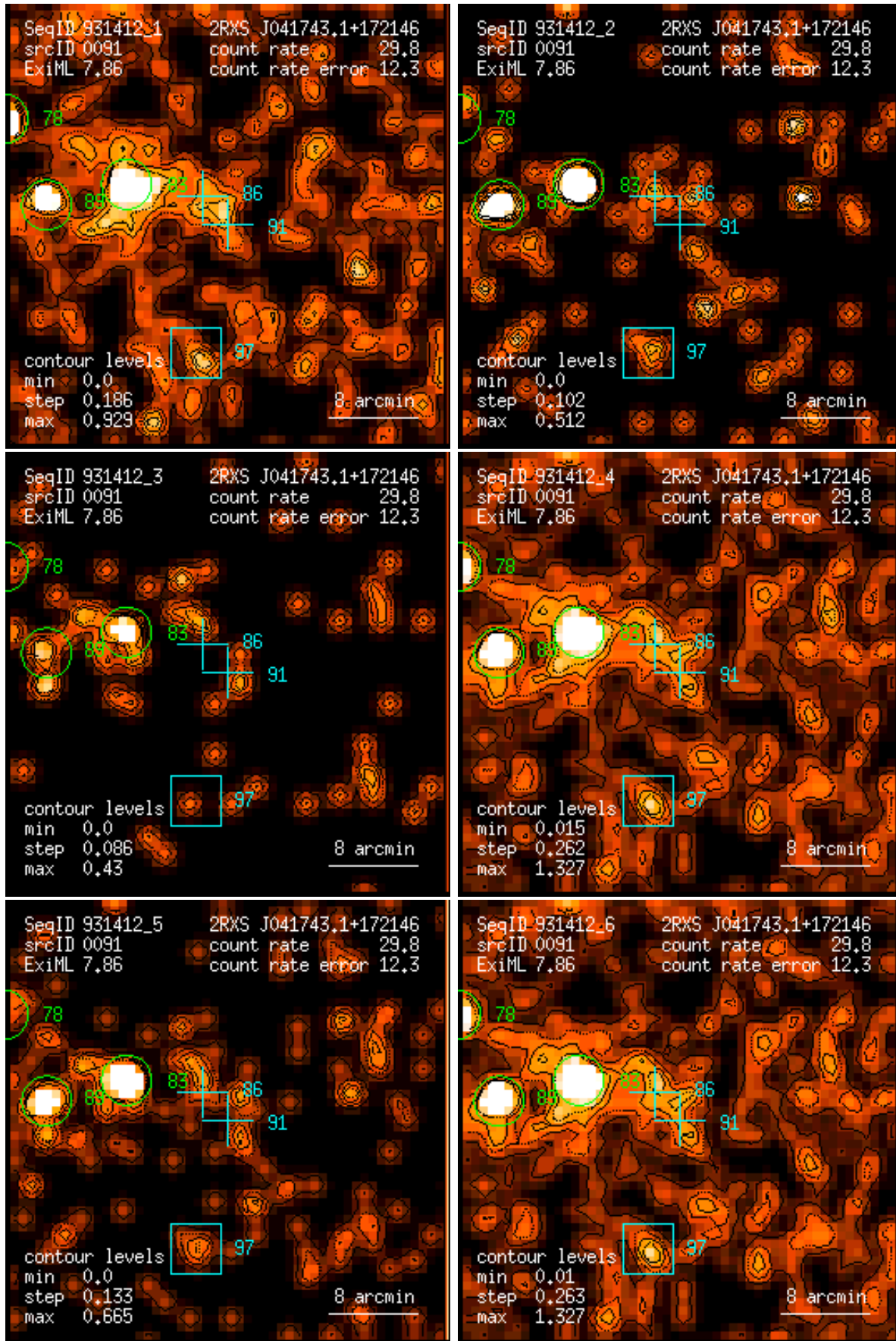
Figure 91: RASS 931412: detection 0091: band rate images, Gaussian filter: (1) PSPC channels 11 – 41, (2) 52 – 90, (3) 91 – 201, (4) 11 – 235, (5) 52 – 201, (6) 11 – 201. Broad band rates in counts/ks. Band rate contour levels in counts/ks/arcmin 2 .
