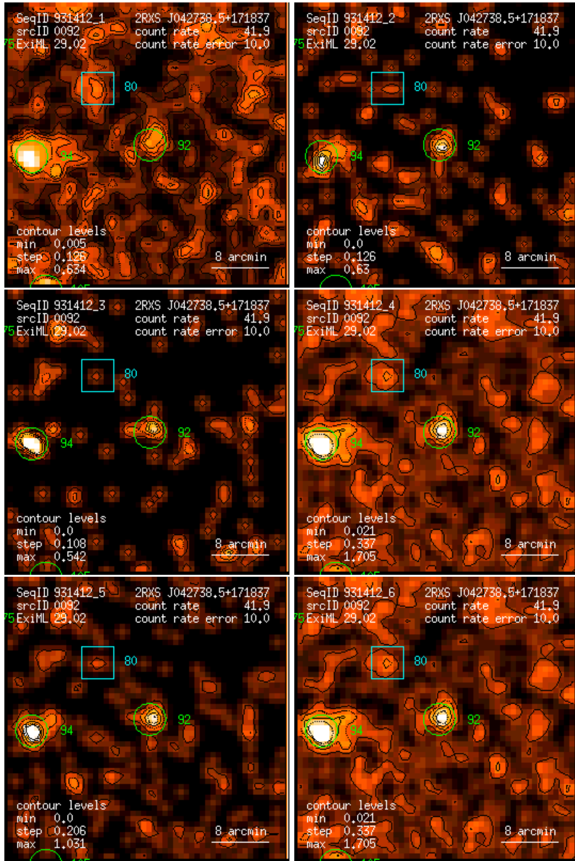
Figure 92: RASS 931412: detection 0092: band rate images, Gaussian filter: (1) PSPC channels 11 – 41, (2) 52 – 90, (3) 91 – 201, (4) 11 – 235, (5) 52 – 201, (6) 11 – 201. Broad band rates in counts/ks. Band rate contour levels in counts/ks/arcmin 2 .
