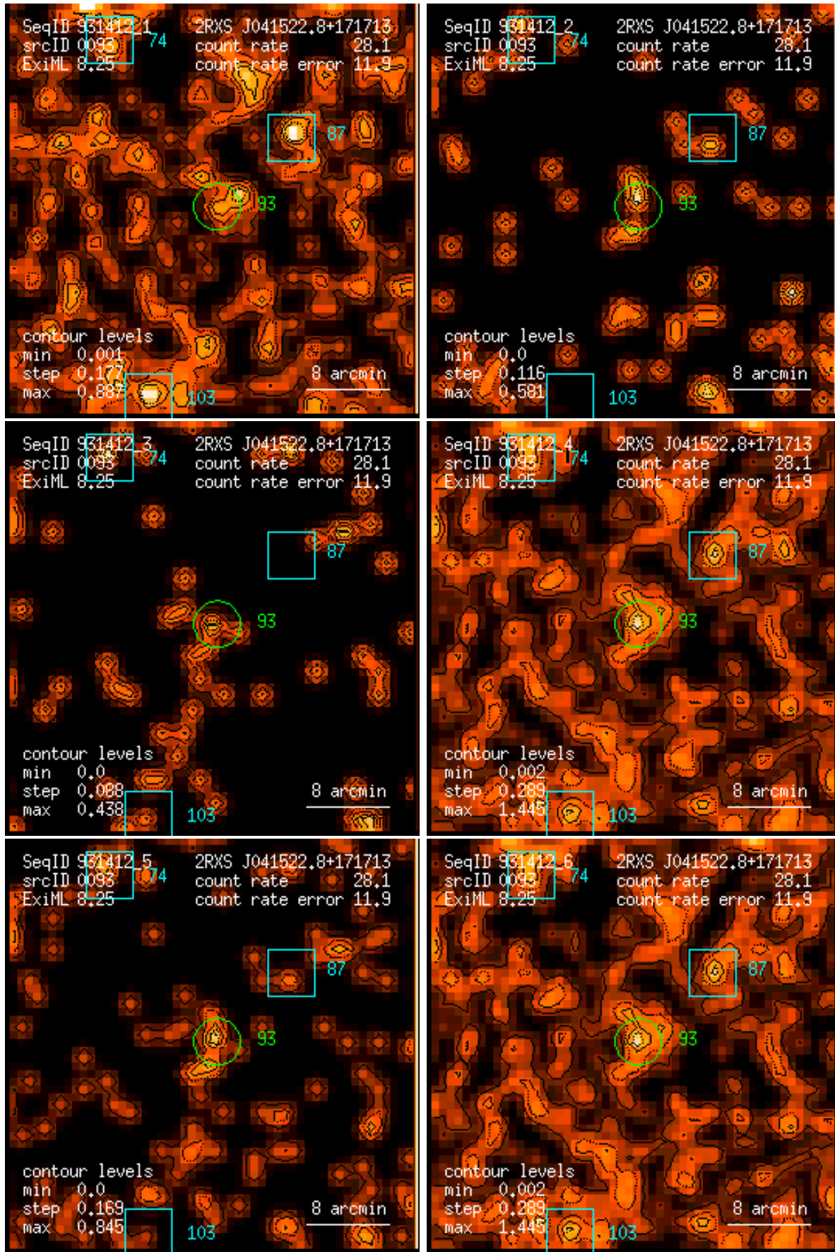
Figure 93: RASS 931412: detection 0093: band rate images, Gaussian filter: (1) PSPC channels 11 – 41, (2) 52 – 90, (3) 91 – 201, (4) 11 – 235, (5) 52 – 201, (6) 11 – 201. Broad band rates in counts/ks. Band rate contour levels in counts/ks/arcmin 2 .
