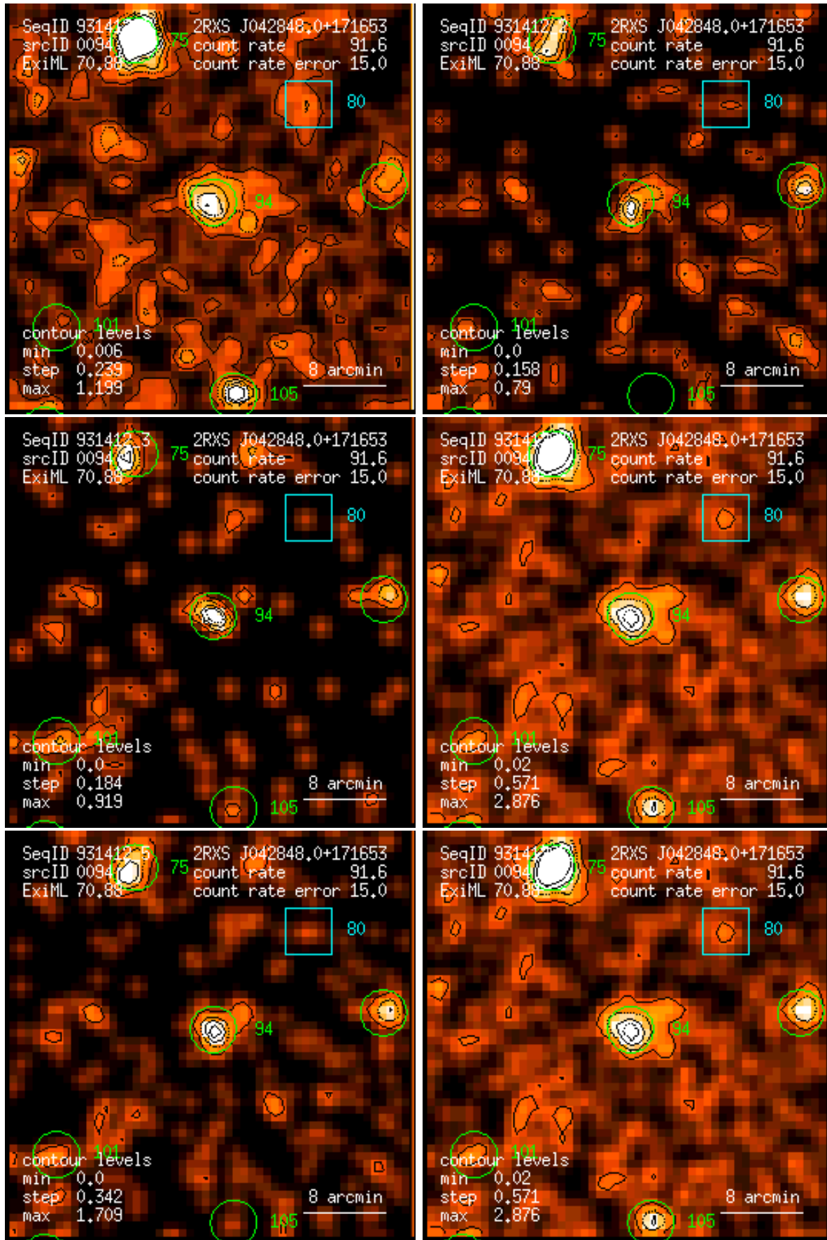
Figure 94: RASS 931412: detection 0094: band rate images, Gaussian filter: (1) PSPC channels 11 – 41, (2) 52 – 90, (3) 91 – 201, (4) 11 – 235, (5) 52 – 201, (6) 11 – 201. Broad band rates in counts/ks. Band rate contour levels in counts/ks/arcmin 2 .
