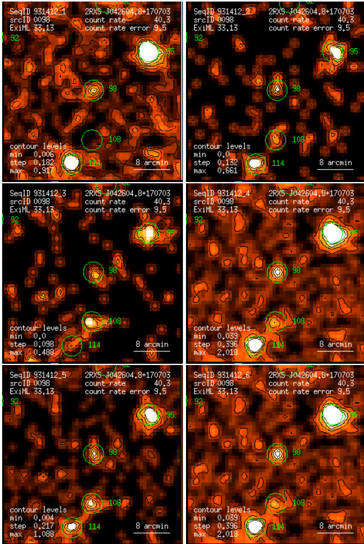
Figure 98: RASS 931412: detection 0098: band rate images, Gaussian filter: (1) PSPC channels 11 – 41, (2) 52 – 90, (3) 91 – 201, (4) 11 – 235, (5) 52 – 201, (6) 11 – 201. Broad band rates in counts/ks. Band rate contour levels in counts/ks/arcmin 2 .
