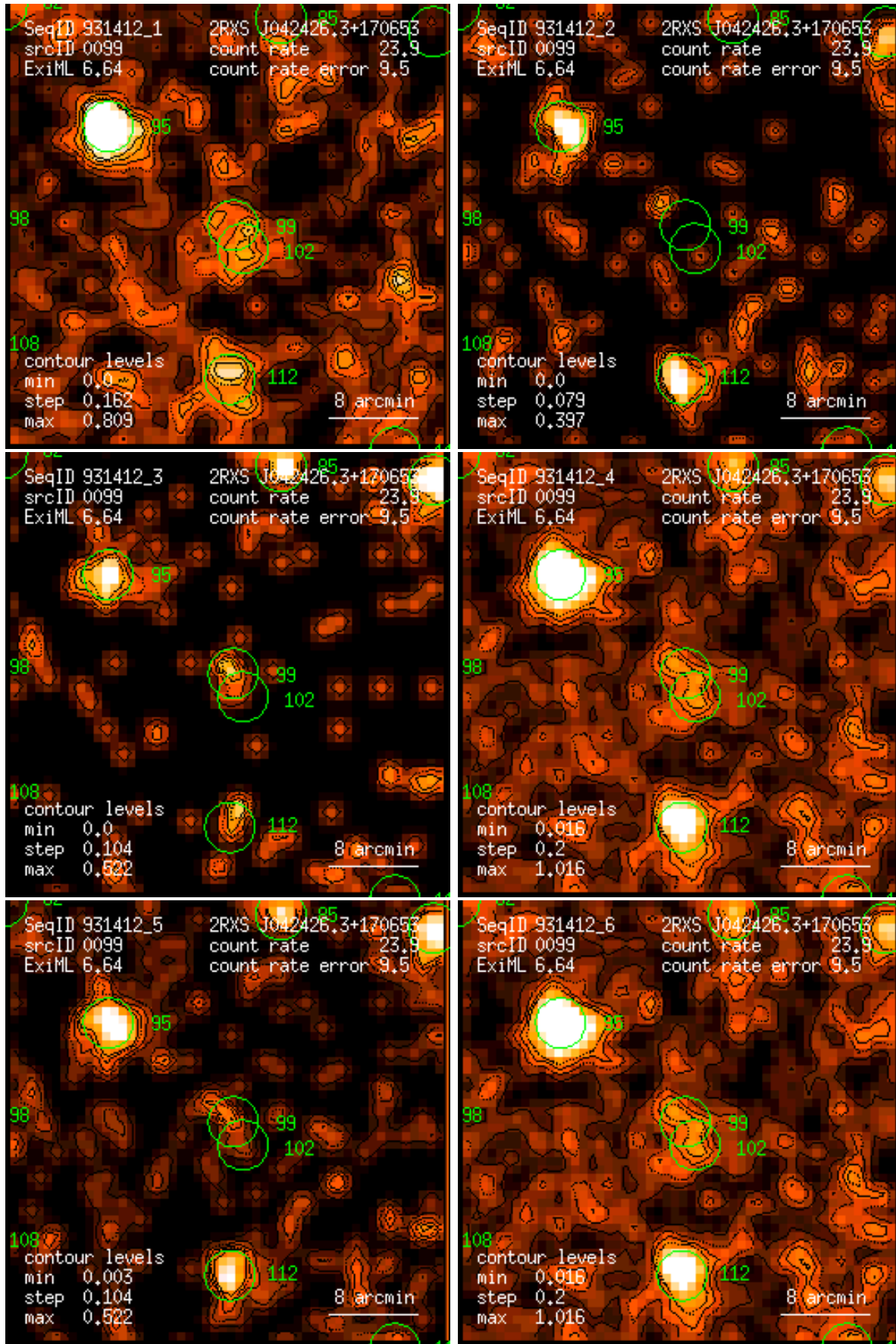
Figure 99: RASS 931412: detection 0099: band rate images, Gaussian filter: (1) PSPC channels 11 – 41, (2) 52 – 90, (3) 91 – 201, (4) 11 – 235, (5) 52 – 201, (6) 11 – 201. Broad band rates in counts/ks. Band rate contour levels in counts/ks/arcmin 2 .
