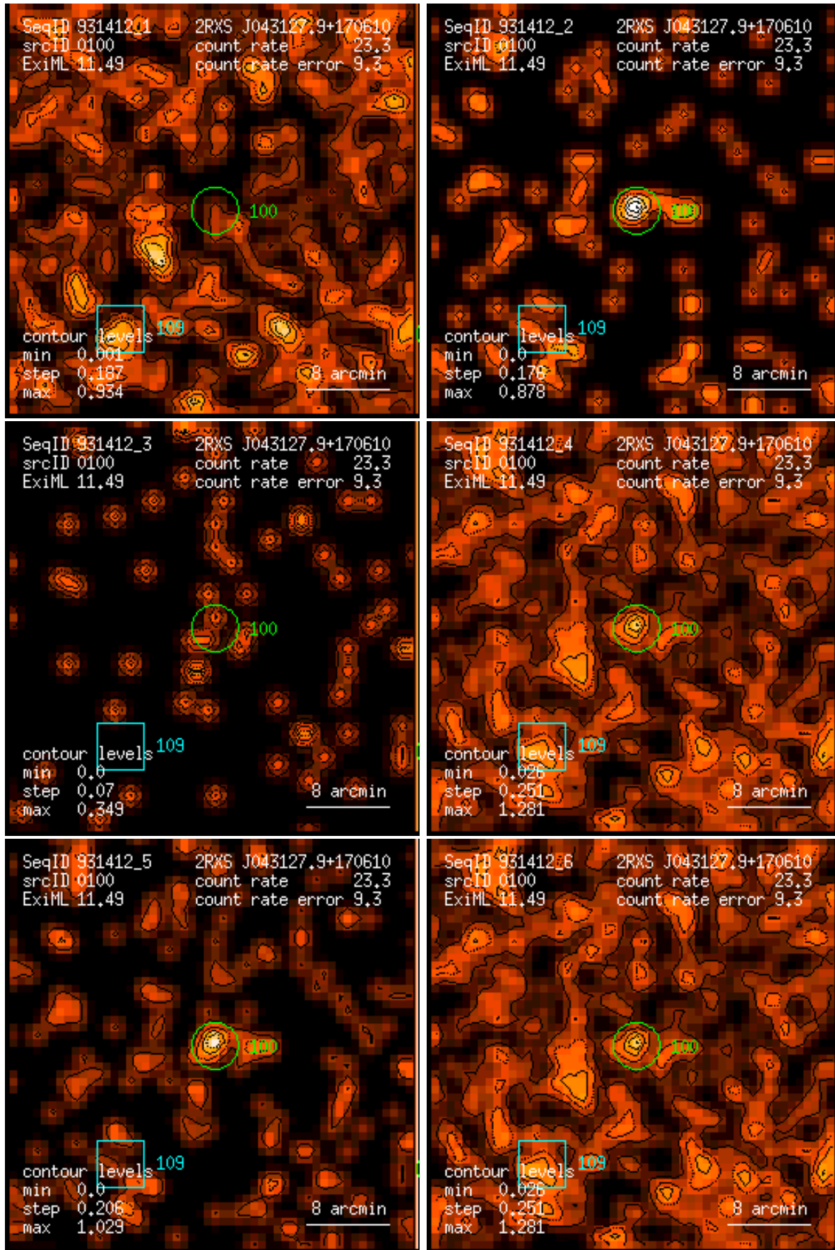
Figure 100: RASS 931412: detection 0100: band rate images, Gaussian filter: (1) PSPC channels 11 – 41, (2) 52 – 90, (3) 91 – 201, (4) 11 – 235, (5) 52 – 201, (6) 11 – 201. Broad band rates in counts/ks. Band rate contour levels in counts/ks/arcmin 2 .
