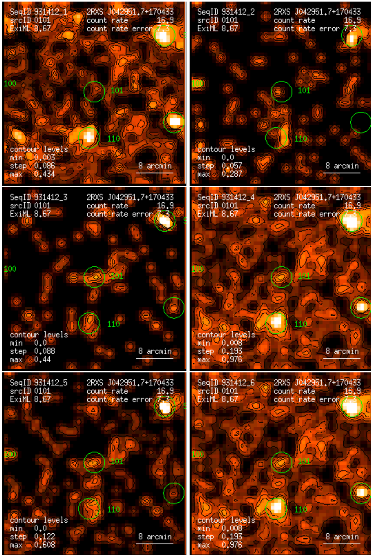
Figure 101: RASS 931412: detection 0101: band rate images, Gaussian filter: (1) PSPC channels 11 – 41, (2) 52 – 90, (3) 91 – 201, (4) 11 – 235, (5) 52 – 201, (6) 11 – 201. Broad band rates in counts/ks. Band rate contour levels in counts/ks/arcmin 2 .
