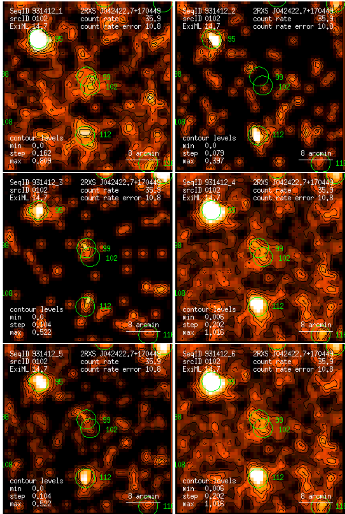
Figure 102: RASS 931412: detection 0102: band rate images, Gaussian filter: (1) PSPC channels 11 – 41, (2) 52 – 90, (3) 91 – 201, (4) 11 – 235, (5) 52 – 201, (6) 11 – 201. Broad band rates in counts/ks. Band rate contour levels in counts/ks/arcmin 2 .
