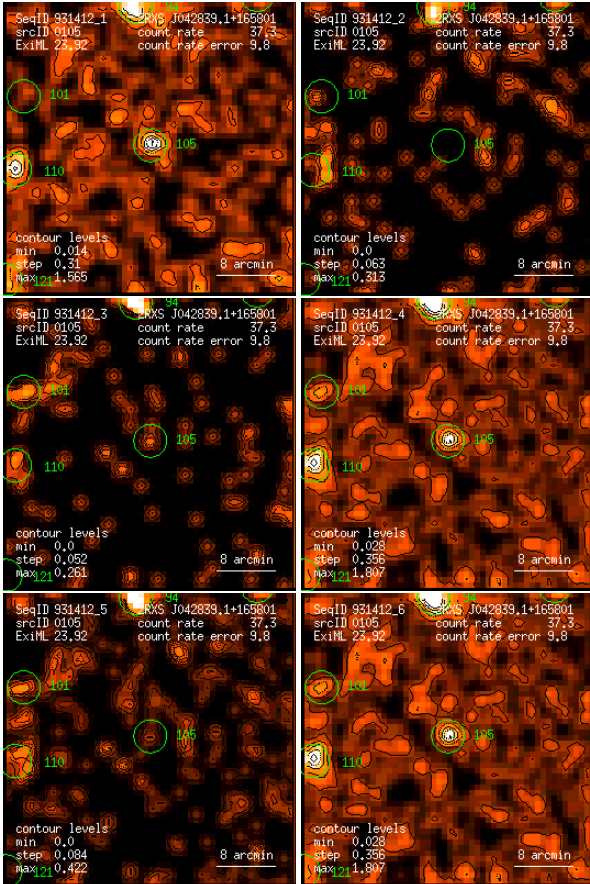
Figure 105: RASS 931412: detection 0105: band rate images, Gaussian filter: (1) PSPC channels 11 – 41, (2) 52 – 90, (3) 91 – 201, (4) 11 – 235, (5) 52 – 201, (6) 11 – 201. Broad band rates in counts/ks. Band rate contour levels in counts/ks/arcmin 2 .
