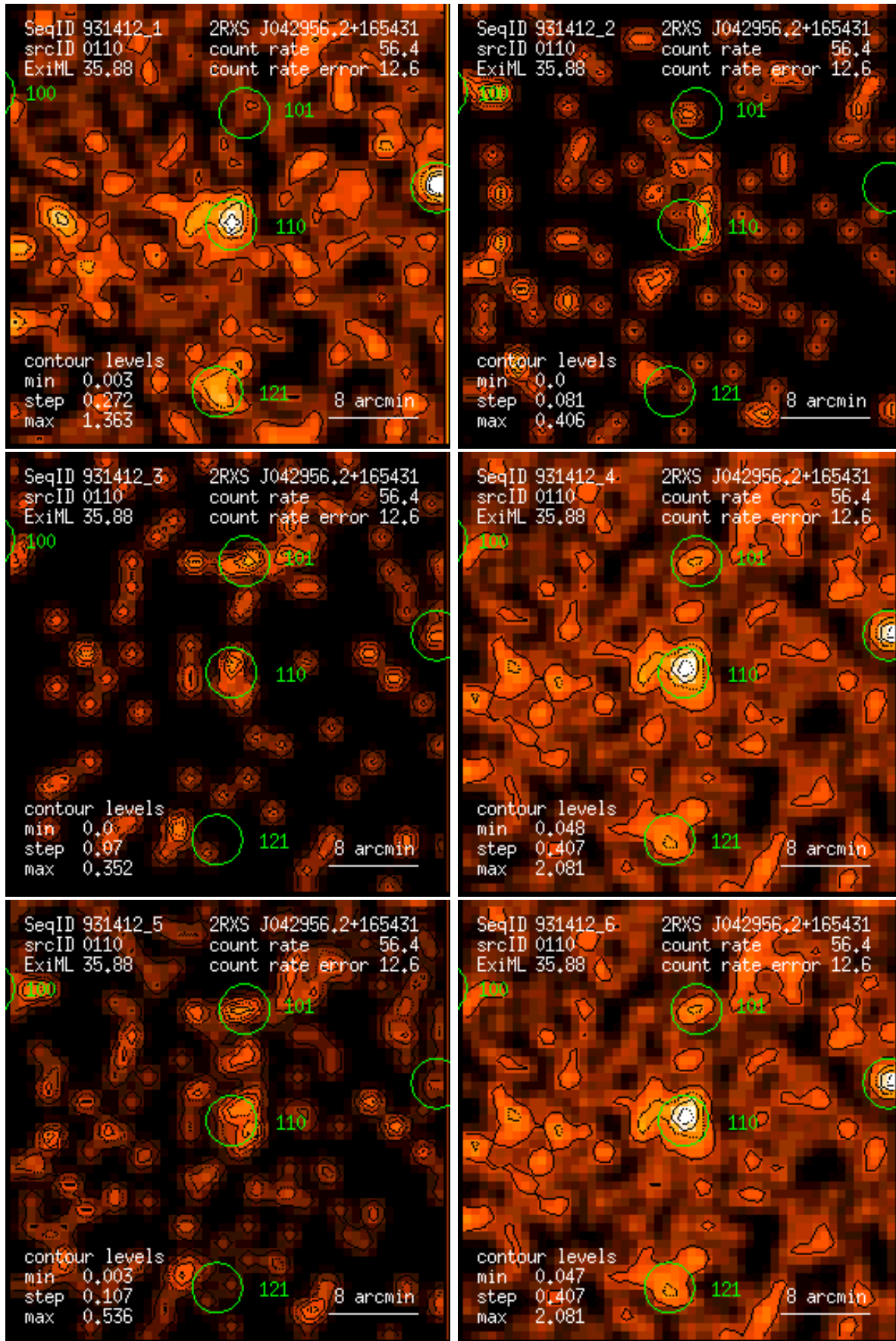
Figure 110: RASS 931412: detection 0110: band rate images, Gaussian filter: (1) PSPP channels 11 – 41, (2) 52 – 90, (3) 91 – 201, (4) 11 – 235, (5) 52 – 201, (6) 11 – 201. Broad band rates in counts/ks. Band rate contour levels in counts/ks/arcmin 2 .
