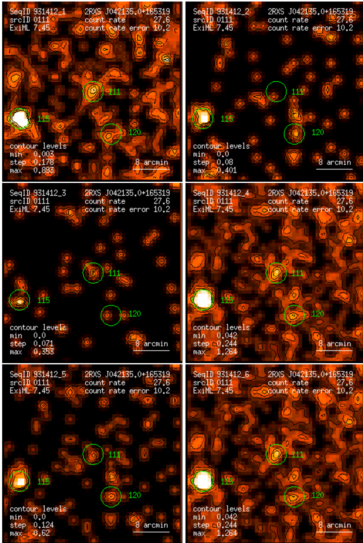
Figure 111: RASS 931412: detection 0111: band rate images, Gaussian filter: (1) PSPC channels 11 – 41, (2) 52 – 90, (3) 91 – 201, (4) 11 – 235, (5) 52 – 201, (6) 11 – 201. Broad band rates in counts/ks. Band rate contour levels in counts/ks/arcmin 2 .
