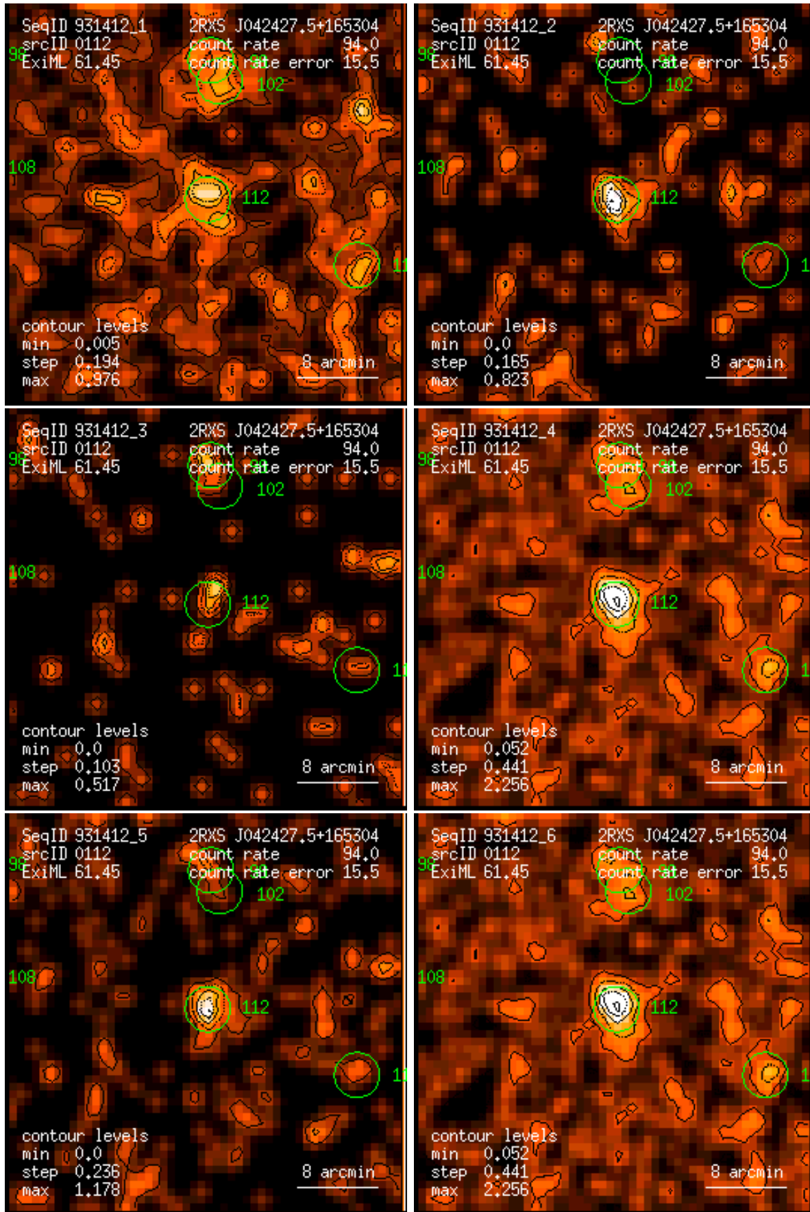
Figure 112: RASS 931412: detection 0112: band rate images, Gaussian filter: (1) PSPC channels 11 – 41, (2) 52 – 90, (3) 91 – 201, (4) 11 – 235, (5) 52 – 201, (6) 11 – 201. Broad band rates in counts/ks. Band rate contour levels in counts/ks/arcmin 2 .
