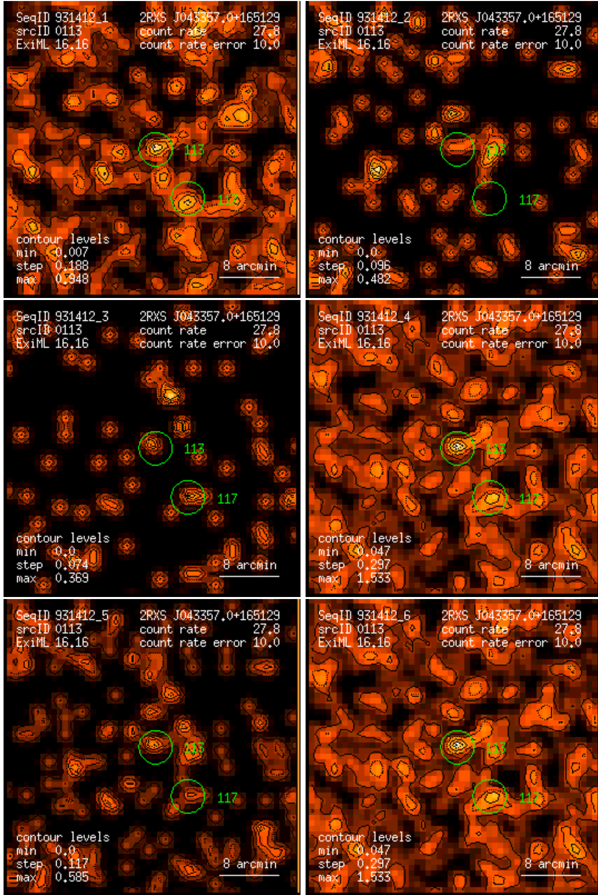
Figure 113: RASS 931412: detection 0113: band rate images, Gaussian filter: (1) PSPC channels 11 – 41, (2) 52 – 90, (3) 91 – 201, (4) 11 – 235, (5) 52 – 201, (6) 11 – 201. Broad band rates in counts/ks. Band rate contour levels in counts/ks/arcmin 2 .
