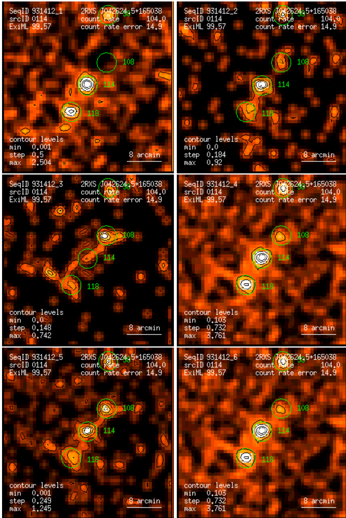
Figure 114: RASS 931412: detection 0114: band rate images, Gaussian filter: (1) PSPC channels 11 – 41, (2) 52 – 90, (3) 91 – 201, (4) 11 – 235, (5) 52 – 201, (6) 11 – 201. Broad band rates in counts/ks. Band rate contour levels in counts/ks/arcmin 2 .
