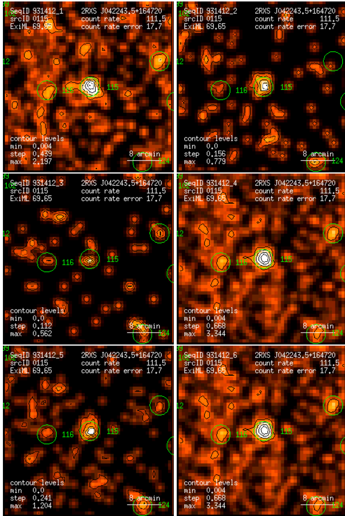
Figure 115: RASS 931412: detection 0115: band rate images, Gaussian filter: (1) PSPC channels 11 – 41, (2) 52 – 90, (3) 91 – 201, (4) 11 – 235, (5) 52 – 201, (6) 11 – 201. Broad band rates in counts/ks. Band rate contour levels in counts/ks/arcmin 2 .
