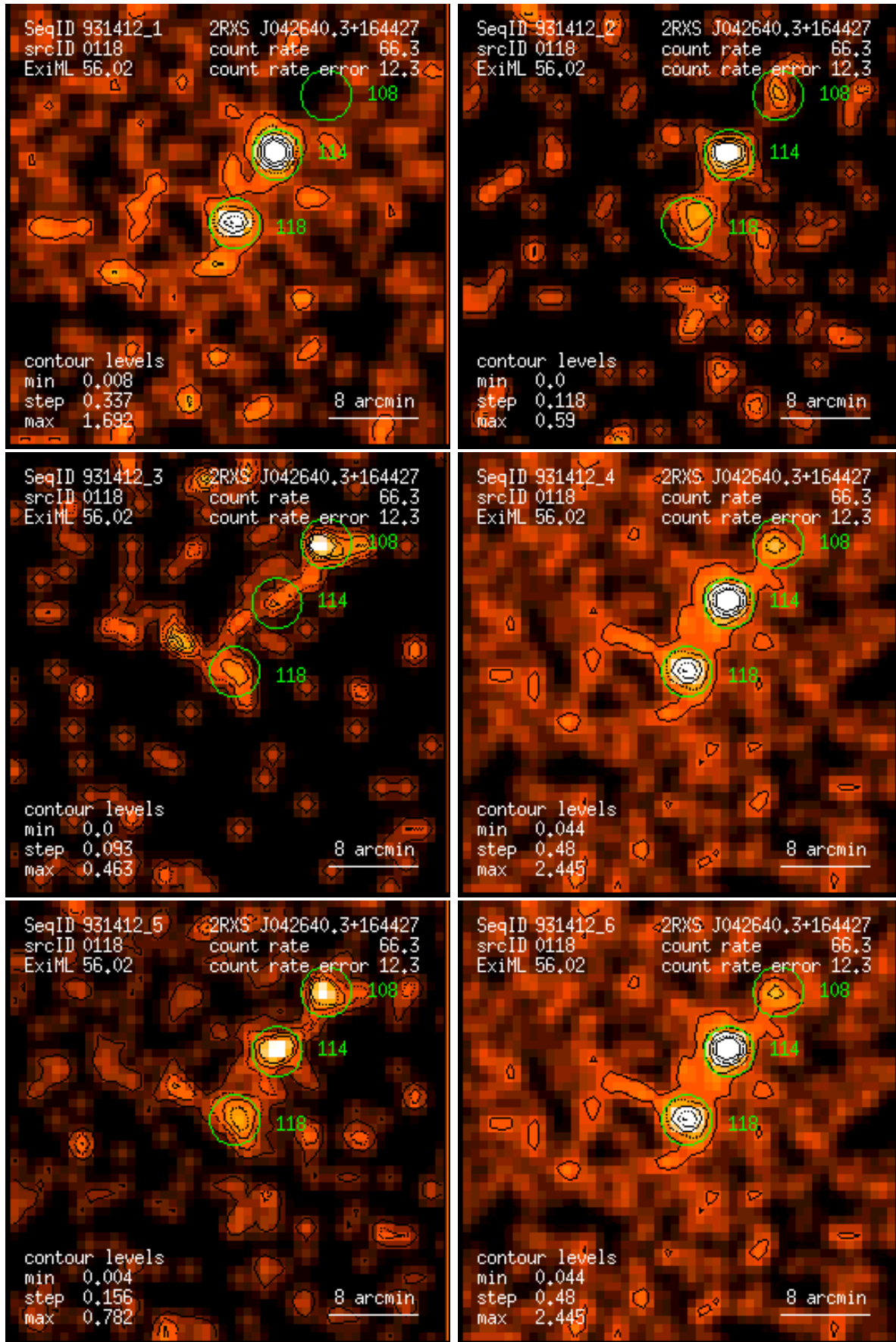
Figure 118: RASS 931412: detection 0118: band rate images, Gaussian filter: (1) PSPC channels 11 – 41, (2) 52 – 90, (3) 91 – 201, (4) 11 – 235, (5) 52 – 201, (6) 11 – 201. Broad band rates in counts/ks. Band rate contour levels in counts/ks/arcmin 2 .
