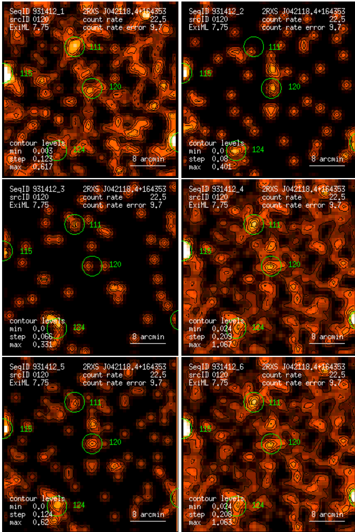
Figure 120: RASS 931412: detection 0120: band rate images, Gaussian filter: (1) PSPC channels 11 – 41, (2) 52 – 90, (3) 91 – 201, (4) 11 – 235, (5) 52 – 201, (6) 11 – 201. Broad band rates in counts/ks. Band rate contour levels in counts/ks/arcmin 2 .
