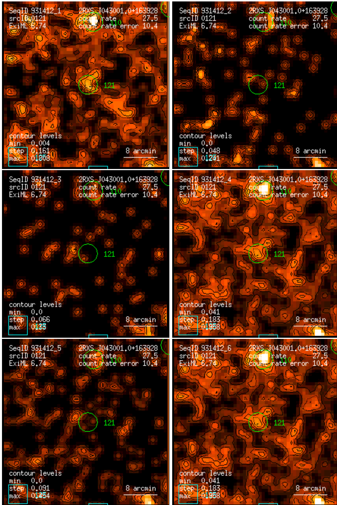
Figure 121: RASS 931412: detection 0121: band rate images, Gaussian filter: (1) PSPC channels 11 – 41, (2) 52 – 90, (3) 91 – 201, (4) 11 – 235, (5) 52 – 201, (6) 11 – 201. Broad band rates in counts/ks. Band rate contour levels in counts/ks/arcmin 2 .
