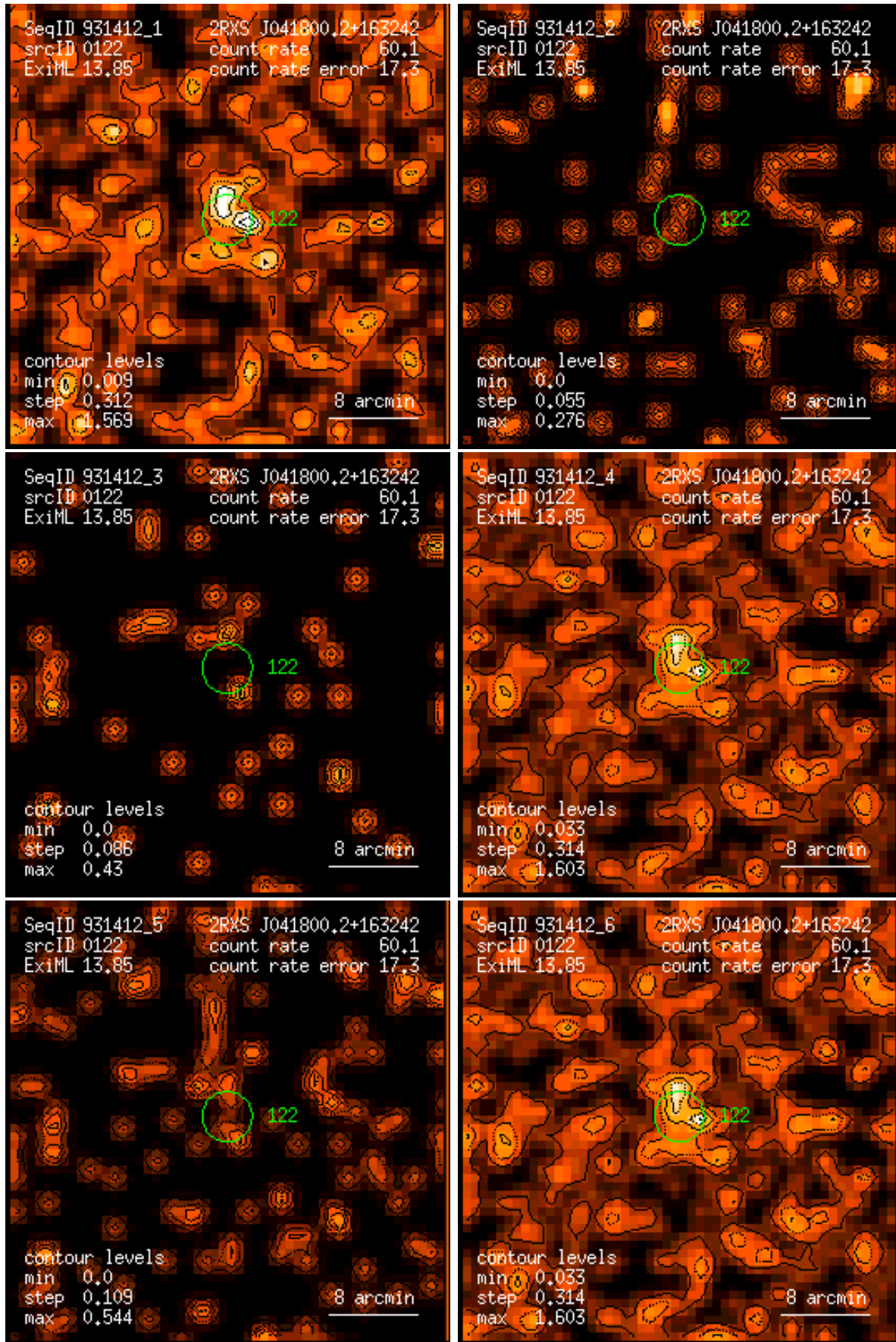
Figure 122: RASS 931412: detection 0122: band rate images, Gaussian filter: (1) PSPC channels 11 – 41, (2) 52 – 90, (3) 91 – 201, (4) 11 – 235, (5) 52 – 201, (6) 11 – 201. Broad band rates in counts/ks. Band rate contour levels in counts/ks/arcmin 2 .
