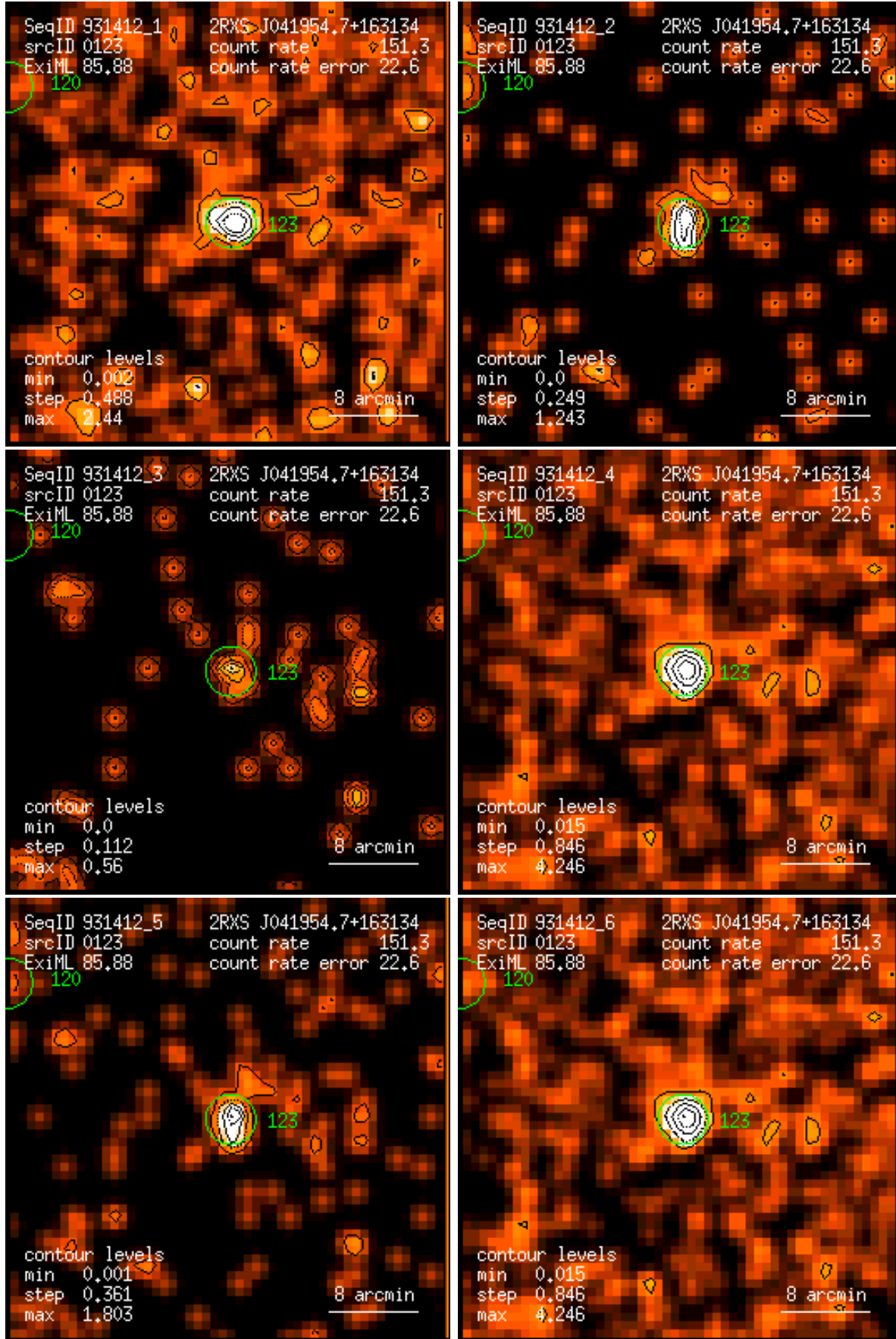
Figure 123: RASS 931412: detection 0123: band rate images, Gaussian filter: (1) PSPC channels 11 – 41, (2) 52 – 90, (3) 91 – 201, (4) 11 – 235, (5) 52 – 201, (6) 11 – 201. Broad band rates in counts/ks. Band rate contour levels in counts/ks/arcmin 2 .
