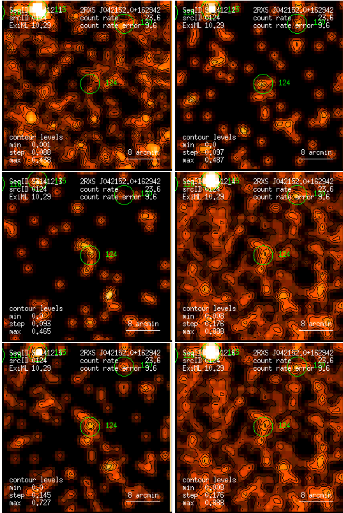
Figure 124: RASS 931412: detection 0124: band rate images, Gaussian filter: (1) PSPC channels 11 – 41, (2) 52 – 90, (3) 91 – 201, (4) 11 – 235, (5) 52 – 201, (6) 11 – 201. Broad band rates in counts/ks. Band rate contour levels in counts/ks/arcmin 2 .
