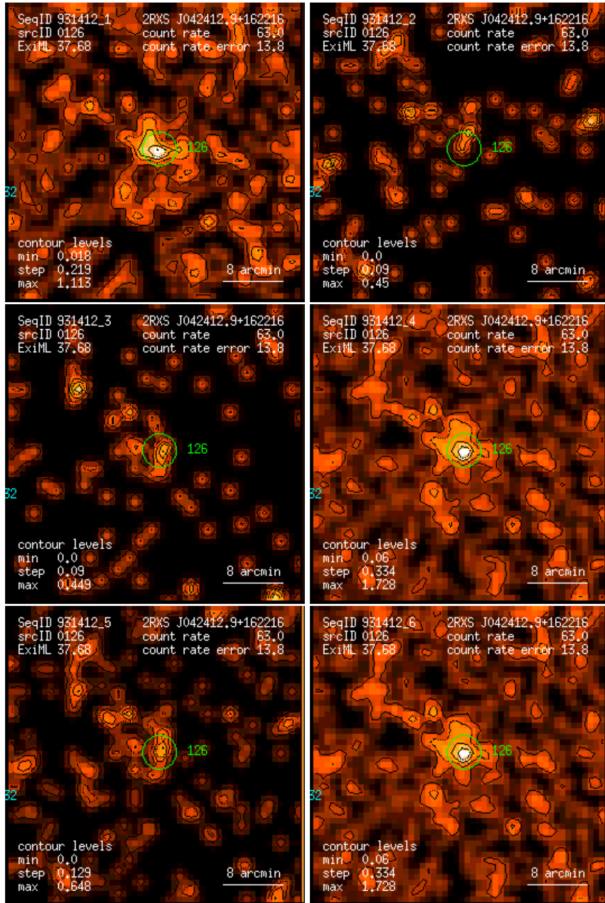
Figure 126: RASS 931412: detection 0126: band rate images, Gaussian filter: (1) PSPC channels 11 – 41, (2) 52 – 90, (3) 91 – 201, (4) 11 – 235, (5) 52 – 201, (6) 11 – 201. Broad band rates in counts/ks. Band rate contour levels in counts/ks/arcmin 2 .
