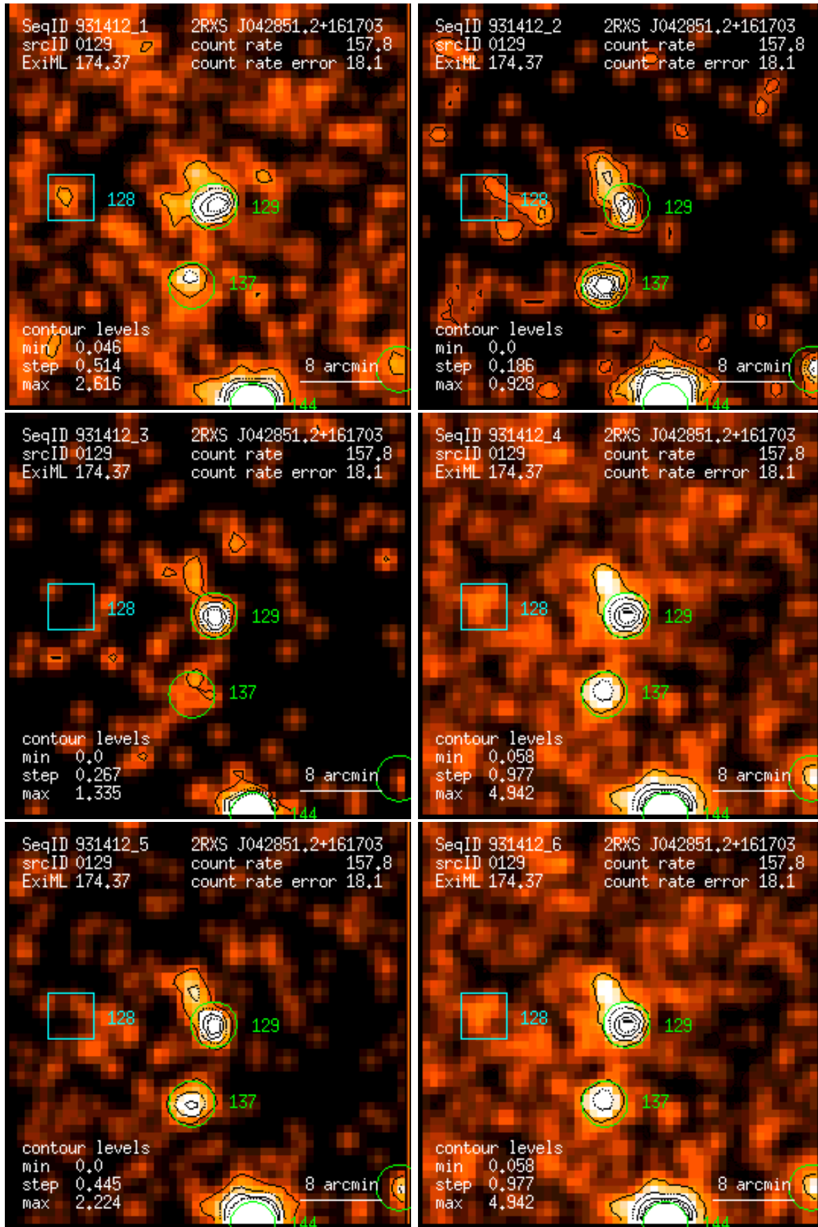
Figure 129: RASS 931412: detection 0129: band rate images, Gaussian filter: (1) PSPC channels 11 – 41, (2) 52 – 90, (3) 91 – 201, (4) 11 – 235, (5) 52 – 201, (6) 11 – 201. Broad band rates in counts/ks. Band rate contour levels in counts/ks/arcmin 2 .
