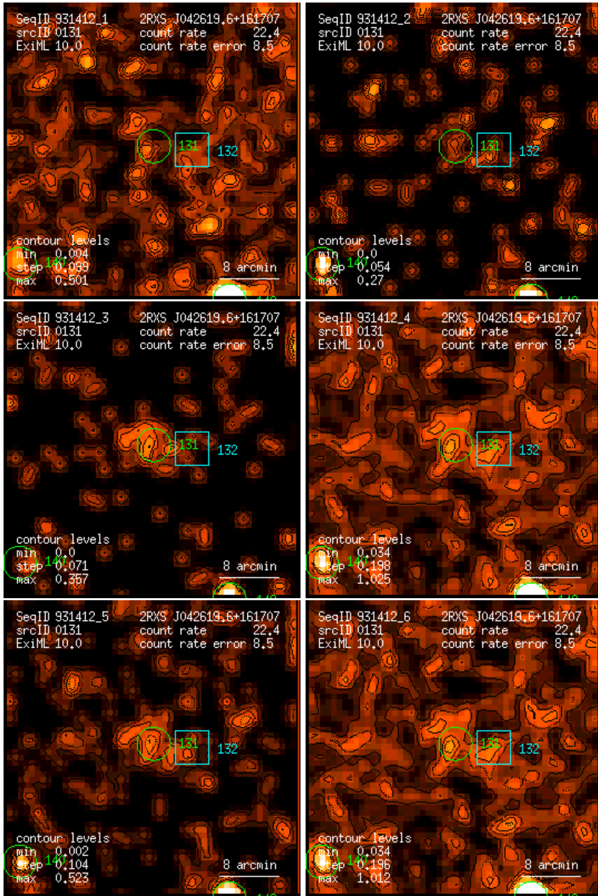
Figure 131: RASS 931412: detection 0131: band rate images, Gaussian filter: (1) PSPC channels 11 – 41, (2) 52 – 90, (3) 91 – 201, (4) 11 – 235, (5) 52 – 201, (6) 11 – 201. Broad band rates in counts/ks. Band rate contour levels in counts/ks/arcmin 2 .
