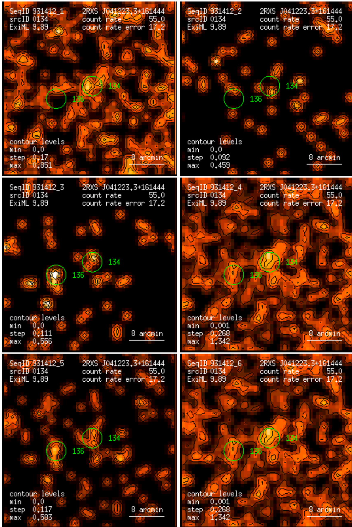
Figure 134: RASS 931412: detection 0134: band rate images, Gaussian filter: (1) PSPC channels 11 – 41, (2) 52 – 90, (3) 91 – 201, (4) 11 – 235, (5) 52 – 201, (6) 11 – 201. Broad band rates in counts/ks. Band rate contour levels in counts/ks/arcmin 2 .
