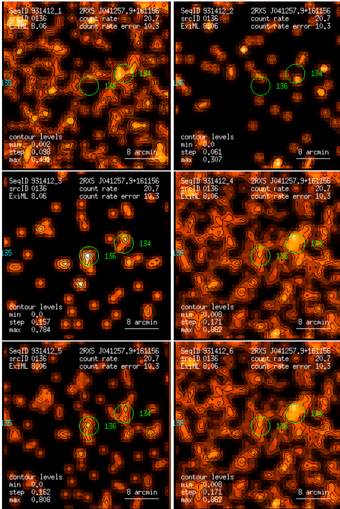
Figure 136: RASS 931412: detection 0136: band rate images, Gaussian filter: (1) PSPC channels 11 – 41, (2) 52 – 90, (3) 91 – 201, (4) 11 – 235, (5) 52 – 201, (6) 11 – 201. Broad band rates in counts/ks. Band rate contour levels in counts/ks/arcmin 2 .
