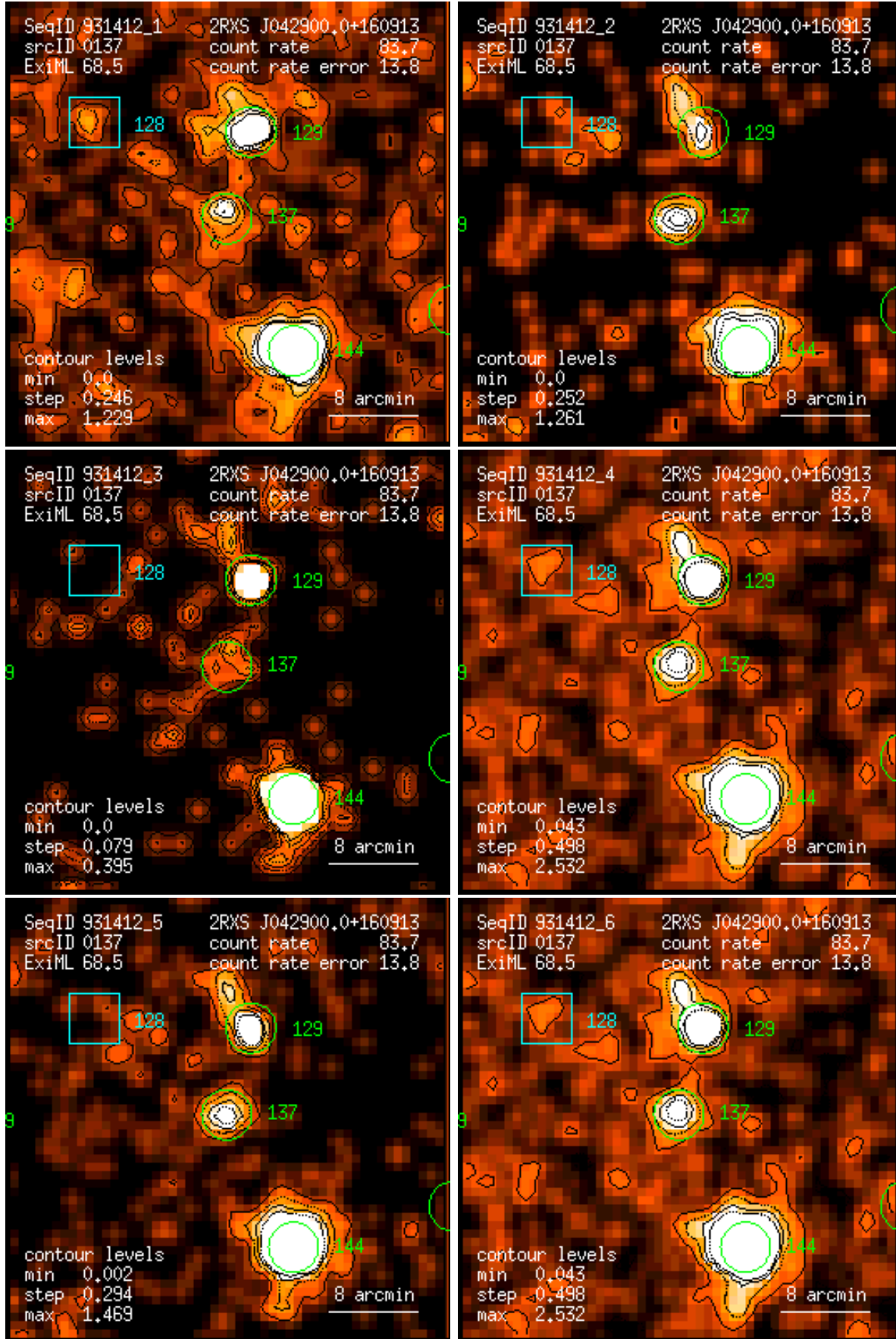
Figure 137: RASS 931412: detection 0137: band rate images, Gaussian filter: (1) PSPC channels 11 – 41, (2) 52 – 90, (3) 91 – 201, (4) 11 – 235, (5) 52 – 201, (6) 11 – 201. Broad band rates in counts/ks. Band rate contour levels in counts/ks/arcmin 2 .
