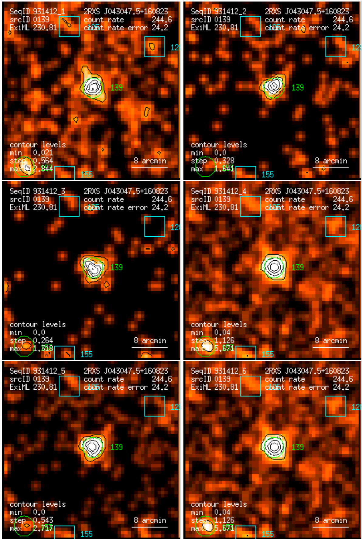
Figure 139: RASS 931412: detection 0139: band rate images, Gaussian filter: (1) PSPC channels 11 – 41, (2) 52 – 90, (3) 91 – 201, (4) 11 – 235, (5) 52 – 201, (6) 11 – 201. Broad band rates in counts/ks. Band rate contour levels in counts/ks/arcmin 2 .
