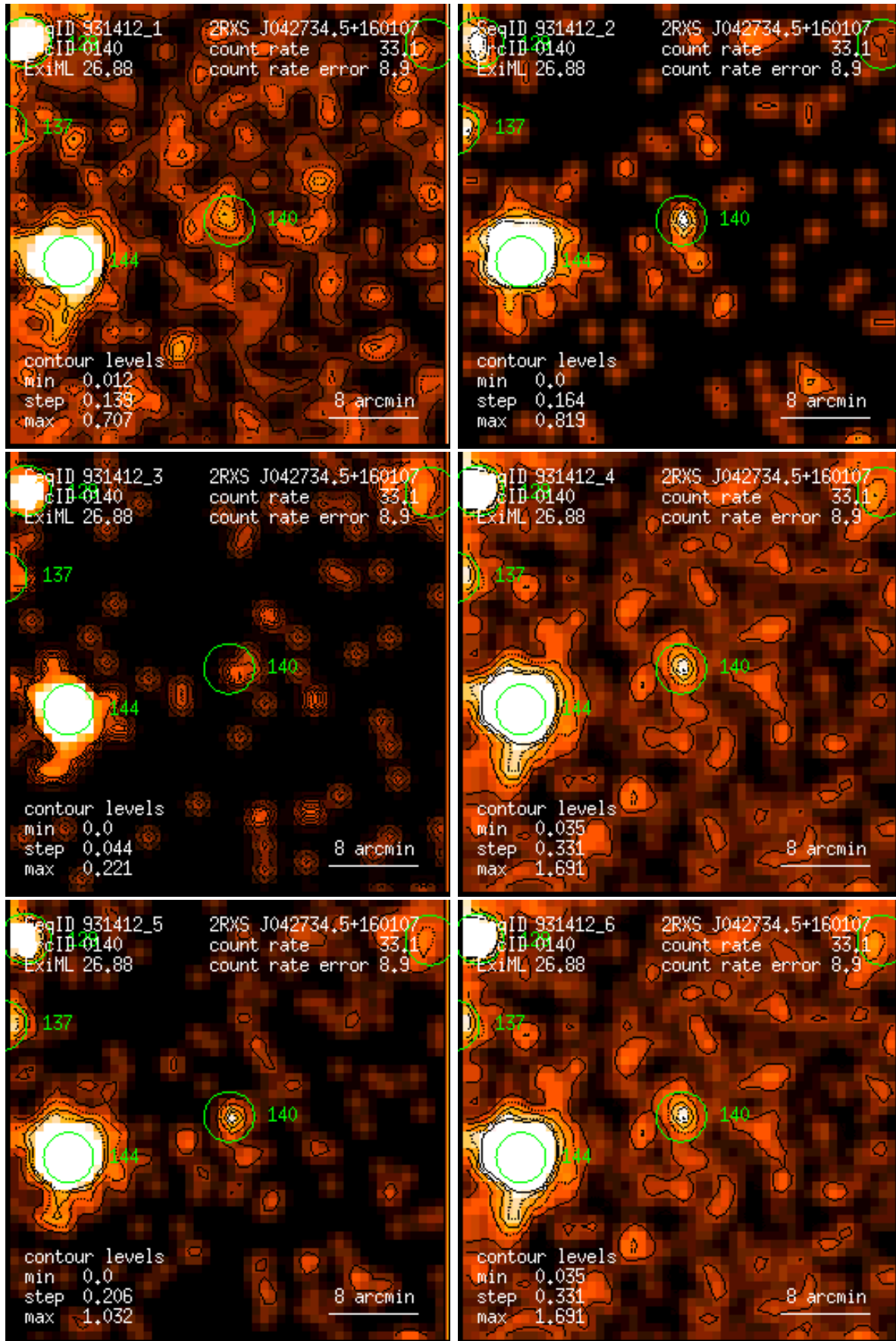
Figure 140: RASS 931412: detection 0140: band rate images, Gaussian filter: (1) PSPC channels 11 – 41, (2) 52 – 90, (3) 91 – 201, (4) 11 – 235, (5) 52 – 201, (6) 11 – 201. Broad band rates in counts/ks. Band rate contour levels in counts/ks/arcmin 2 .
