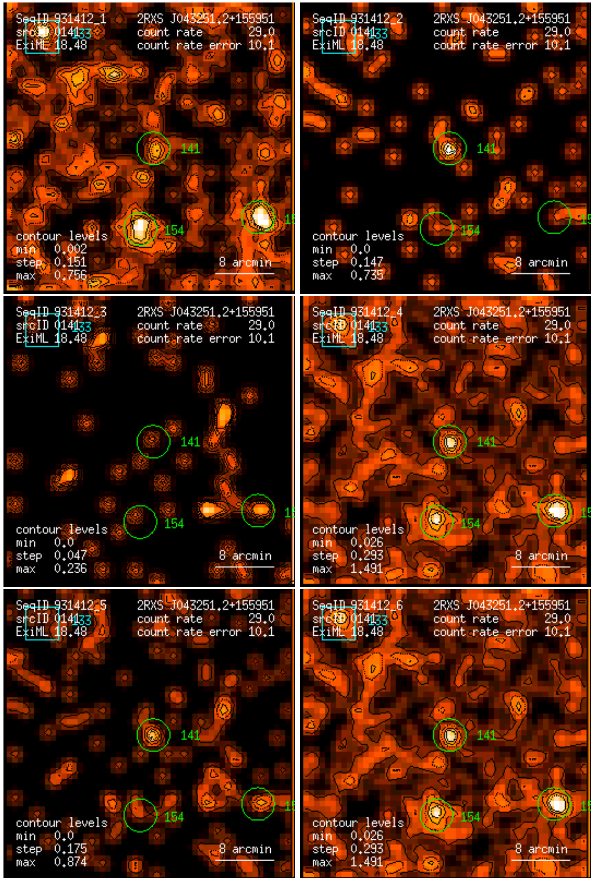
Figure 141: RASS 931412: detection 0141: band rate images, Gaussian filter: (1) PSPC channels 11 – 41, (2) 52 – 90, (3) 91 – 201, (4) 11 – 235, (5) 52 – 201, (6) 11 – 201. Broad band rates in counts/ks. Band rate contour levels in counts/ks/arcmin 2 .
