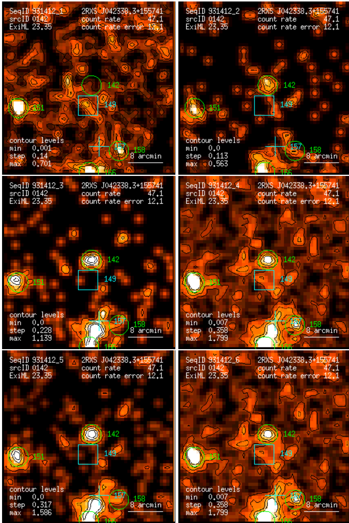
Figure 142: RASS 931412: detection 0142: band rate images, Gaussian filter: (1) PSPC channels 11 – 41, (2) 52 – 90, (3) 91 – 201, (4) 11 – 235, (5) 52 – 201, (6) 11 – 201. Broad band rates in counts/ks. Band rate contour levels in counts/ks/arcmin 2 .
