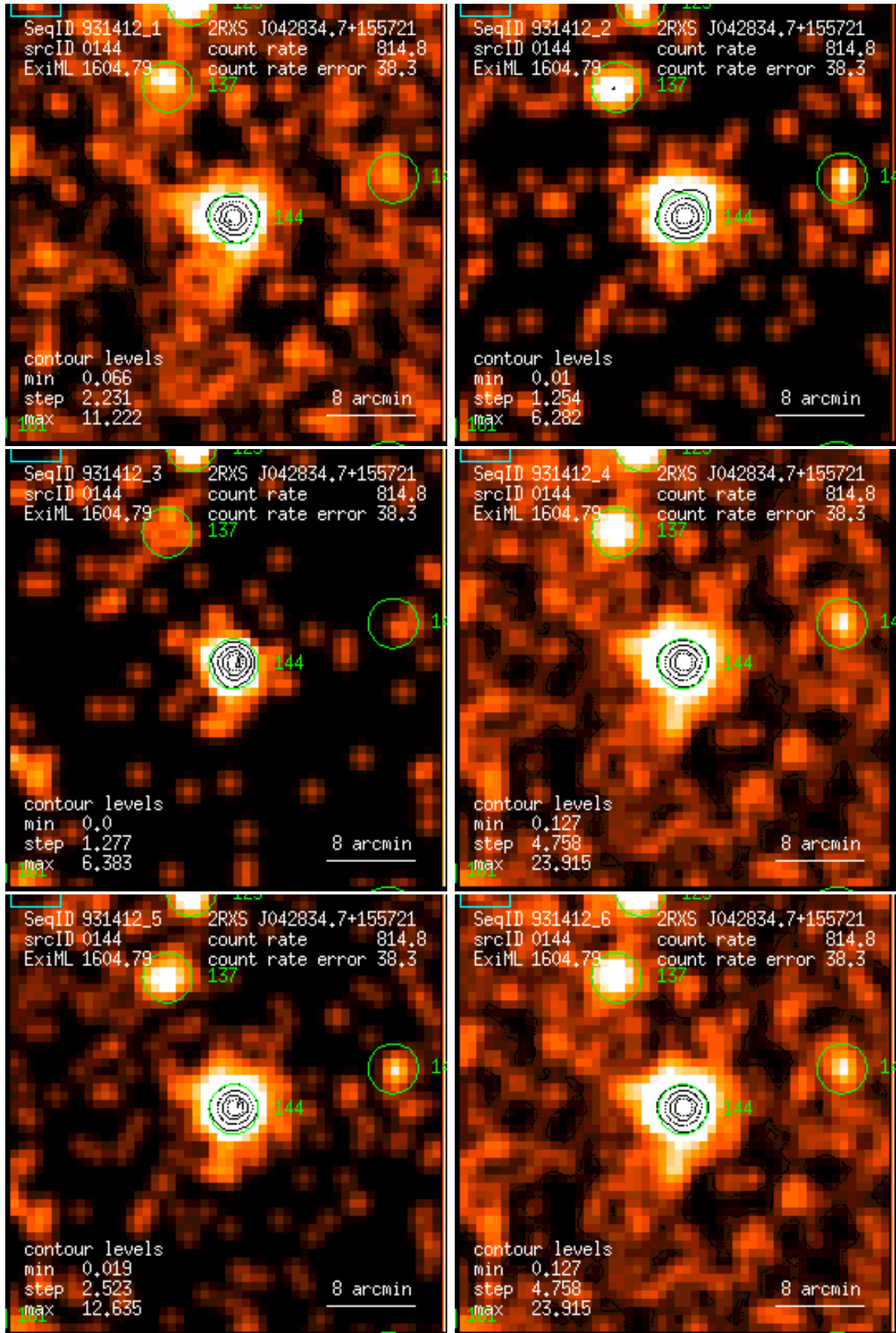
Figure 144: RASS 931412: detection 0144: band rate images, Gaussian filter: (1) PSPC channels 11 – 41, (2) 52 – 90, (3) 91 – 201, (4) 11 – 235, (5) 52 – 201, (6) 11 – 201. Broad band rates in counts/ks. Band rate contour levels in counts/ks/arcmin 2 .
