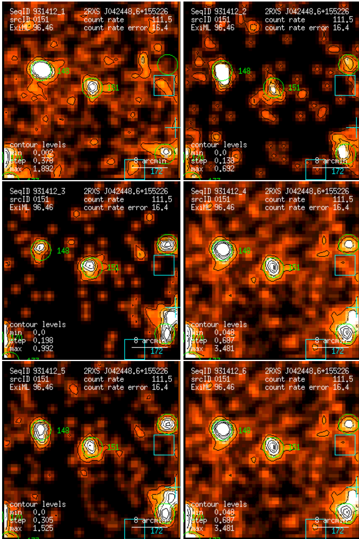
Figure 151: RASS 931412: detection 0151: band rate images, Gaussian filter: (1) PSPC channels 11 – 41, (2) 52 – 90, (3) 91 – 201, (4) 11 – 235, (5) 52 – 201, (6) 11 – 201. Broad band rates in counts/ks. Band rate contour levels in counts/ks/arcmin 2 .
