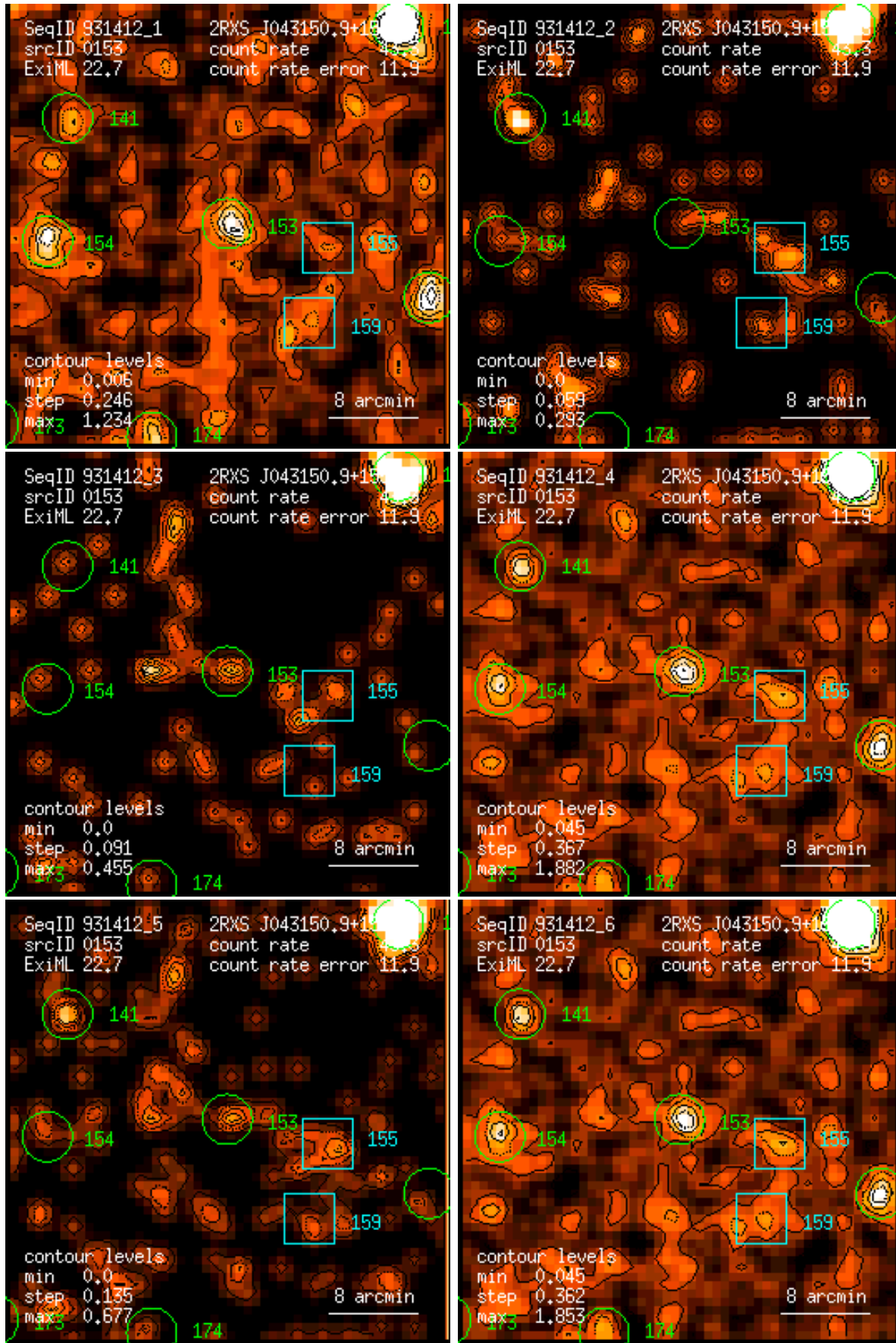
Figure 153: RASS 931412: detection 0153: band rate images, Gaussian filter: (1) PSPC channels 11 – 41, (2) 52 – 90, (3) 91 – 201, (4) 11 – 235, (5) 52 – 201, (6) 11 – 201. Broad band rates in counts/ks. Band rate contour levels in counts/ks/arcmin 2 .
