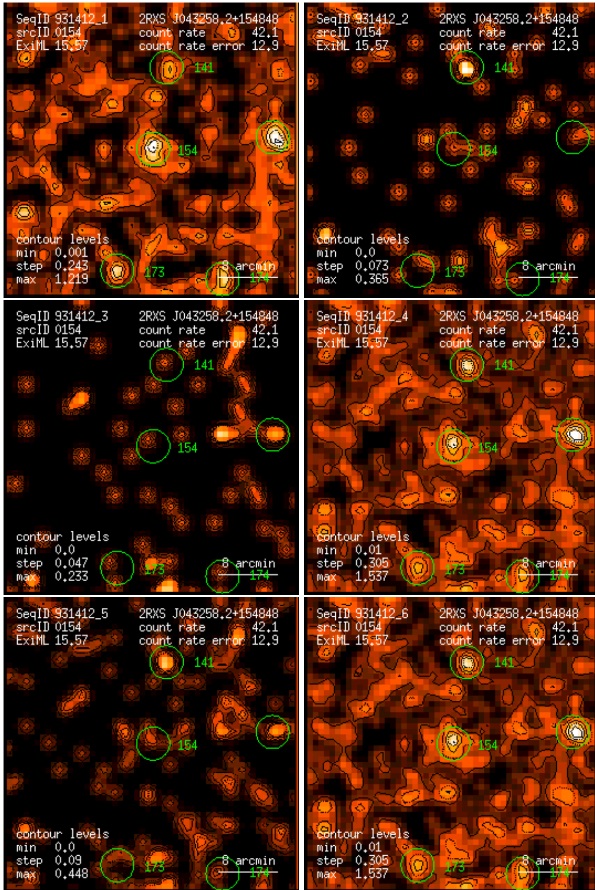
Figure 154: RASS 931412: detection 0154: band rate images, Gaussian filter: (1) PSPC channels 11 – 41, (2) 52 – 90, (3) 91 – 201, (4) 11 – 235, (5) 52 – 201, (6) 11 – 201. Broad band rates in counts/ks. Band rate contour levels in counts/ks/arcmin 2 .
