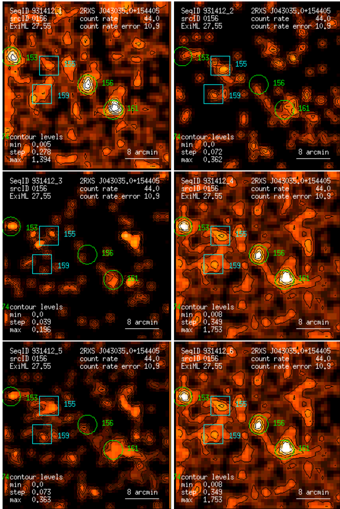
Figure 156: RASS 931412: detection 0156: band rate images, Gaussian filter: (1) PSPC channels 11 – 41, (2) 52 – 90, (3) 91 – 201, (4) 11 – 235, (5) 52 – 201, (6) 11 – 201. Broad band rates in counts/ks. Band rate contour levels in counts/ks/arcmin 2 .
